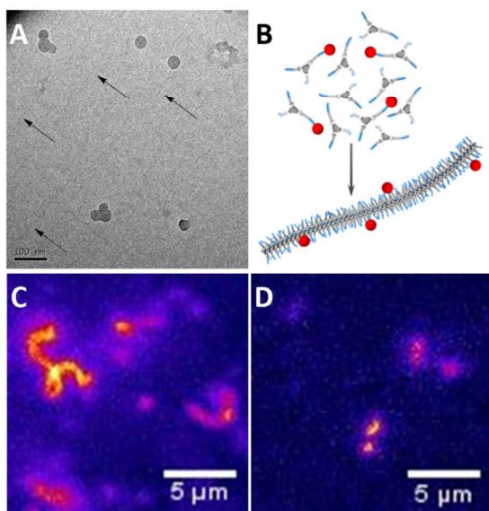
Figure 2. A) CryoTEM image of 1b (0.5 mg/mL) in H 2 O revealing the presence of supramolecular polymers. B) Schematic representation of mixing a small amount of dye labelled BTAs with unlabelled BTAs prior to injection into water, to allow the assembly of the BTAs into fluorescently labelled fibres. Snapshots from movies taken during fluorescence microscopy (samples were equilibrated at 1 \times 10^{-5} M, and diluted to 1 \times 10^{-6} M prior to imaging. See ESI for sample preparation) show C) fibres formed by 1a with 5% 3a and D) fibres formed by 1b with 5% 3b with lengths close to the resolution limit.
