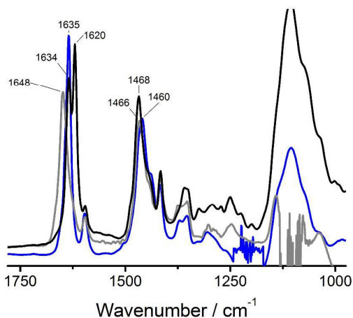
Figure 4. FT-IR spectrum of 1a-d6 in the bulk at 25 °C (black), FT-IR spectrum of a solution of 1a ( c = 50 mg/mL) at room temperature in D 2 O (blue) displaying an amide I vibration indicative for hydrogen bonding and in MeOD (grey) displaying an amide I vibration indicative for the absence of hydrogen bonding.
