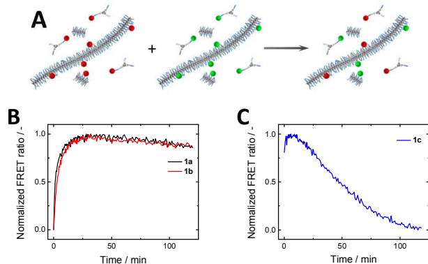
Figure 5. A) Schematic of FRET exchange experiment. B) FRET experiments of 1a and 1b show similar exchange kinetics, while C) 1c shows erratic behaviour due to poor self-assembly. ( c_{BTA} = 1 \times 10^{-5} M)
