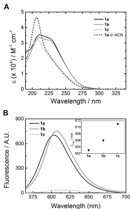
Figure 3. A) UV-vis spectra at 20 °C of 1a , 1b , 1c in H 2 O ( c = 5 \times 10^{-5} M), and 1a in acetonitrile ( c = 1 \times 10^{-5} M) B) Fluorescence emission spectra of Nile Red in solutions of 1a–c in H 2 O ( c_{\text{BTA}} = 1 \times 10^{-5} M, c_{\text{NR}} = 5 \times 10^{-6} M) at 20 °C.
