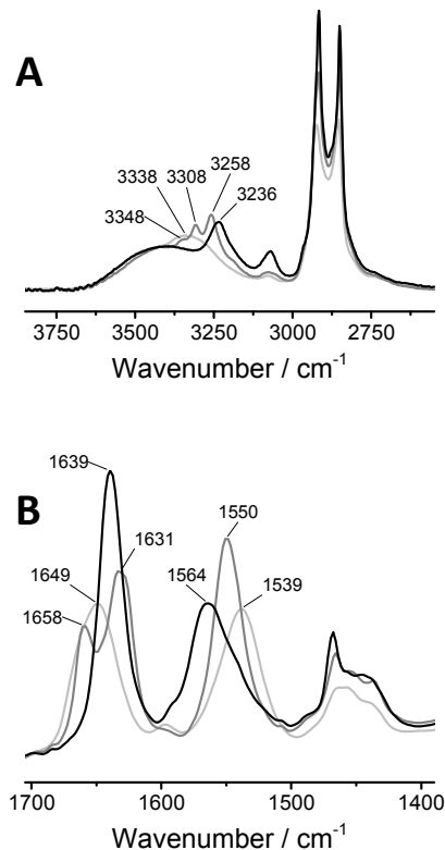
Figure 1. FT-IR spectra of 1a (black curve), 1b (grey curve), and 1c (light grey curve) in the solid state at 25 °C. A) Zoom of the N-H vibration region. B) Zoom of the amide I and amide II region.
