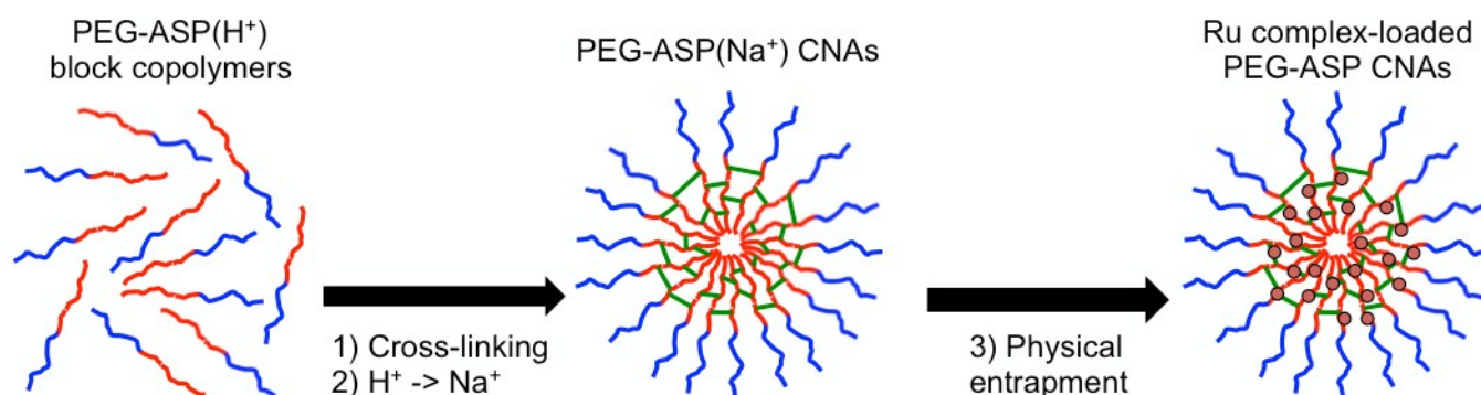
Figure 2: PEG (5k) (blue lines)-ASP (35 units) (red lines) CNA preparation. 1) PEG-ASP(H + ) block copolymers were cross-linked (green lines) with diaminoctane (DAO) activated with diisopropylcarbodiimide (DIC)/ N-hydroxysuccinimide (NHS)/ dimethylaminopyridine (DMAP); 2) ASP(H + ) groups of PEG-ASP CNAs converted to ASP(Na + ); 3) positively charged Ru complexes (red circles) were physically entrapped inside PEG-ASP CNAs through electrostatic interactions with ASP(Na + ) groups.
