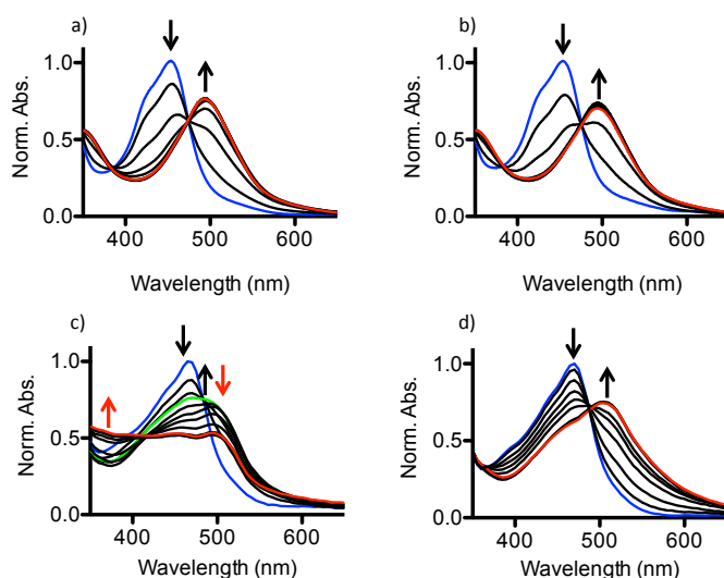
Figure 4: Photoejection kinetics of a) free 1 , b) 1 -loaded PEG-ASP CNAs, c) free 2 , and d) 2 -loaded PEG-ASP CNAs. The blue lines indicate the spectra of initial Ru complex prodrugs, red lines indicate final photoactivated product(s), and the green line in c) indicates a transition between the primary and secondary phases ( t = 90 sec).
