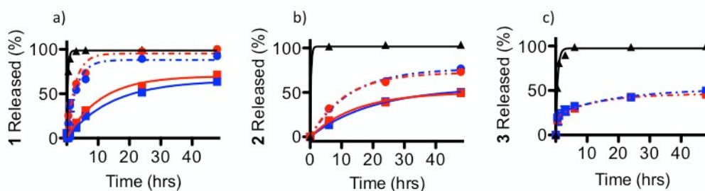
Figure 7: The effect of phosphate buffer pH on complex release from PEG-ASP CNAs through 10K MWCO dialysis cassettes for a) 1 , b) 2 , and c) 3 (dark pH 6.0 (—●—), dark pH 7.4 (—●—), light pH 6.0 (—■—), and light pH 7.4 (—■—)) compared to the release of free complexes from 10K MWCO dialysis cassettes (—▲—) (N = 3). Because 3 was a photostable Ru complex, release was only evaluated when protected from light (N = 3).
