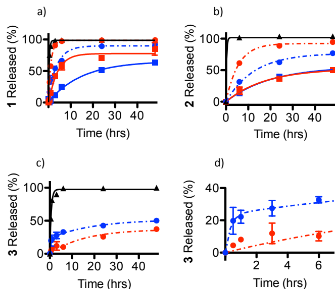
Figure 6: The effect of buffer ionic strength on release from PEG-ASP CNAs for a) 1 , b) 2 , and c) 3 (free complex (▲), dark phosphate buffer (●), dark PBS (●), light phosphate buffer (■), and light PBS (■)); d) shows a magnification of the rapid release of 3 from PEG-ASP CNAs when placed in a solution with low ionic strength (0 mM NaCl) (N = 3). Because 3 was a photostable Ru complex, release was only evaluated when protected from light.
