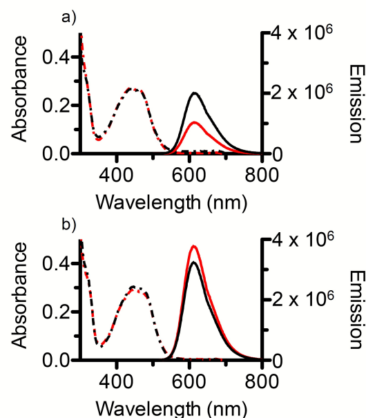
Figure 9: UV/Vis absorbance spectra (hatched lines) and emission spectra (solid lines) in air-equilibrated diH 2 O (red) and deoxygenated (Ar purged) diH 2 O (black) for a) free 3, and b) 3-loaded PEG-ASP CNAs.
