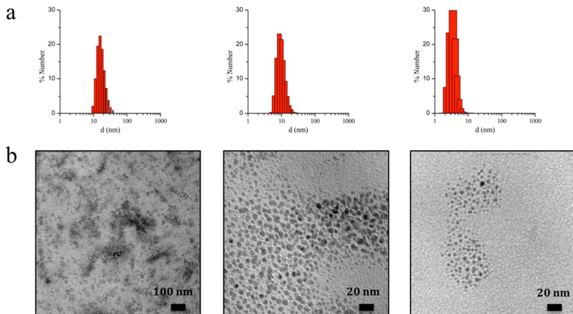
Figure 2. (a) Number-based particle size distribution for the colloidal suspension 1.6 (left), 1.10 (middle) and 1.2 (right) obtained by DLS analysis. (b) TEM images of the same NPs displaying sizes of 16 nm (left), 10 nm (middle) and 4 nm (right) deposited by drop casting on a carbon coated copper grid (left) or placing an ultrathin-section of the dispersed colloids using cryo-microtomy (middle and right).
