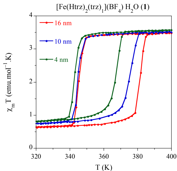
Figure 4. Temperature dependence of the molar magnetic susceptibility temperature product ( \chi_m T ) for samples 1.6 (16 nm), 1.10 (10 nm) and 1.2 (4 nm) after several heating-cooling modes.
