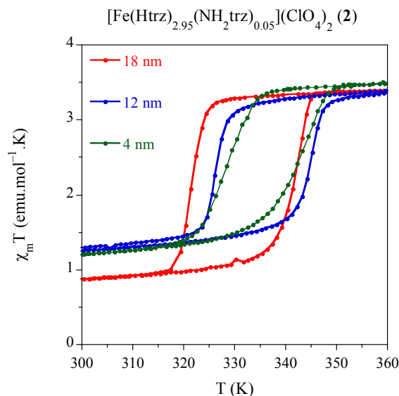
Figure 5. Temperature dependence of the molar magnetic susceptibility temperature product ( \chi_M T ) for samples 2.1 (18 nm), 2.2 (12 nm) and 2.3 (4 nm) after several heating-cooling modes.
