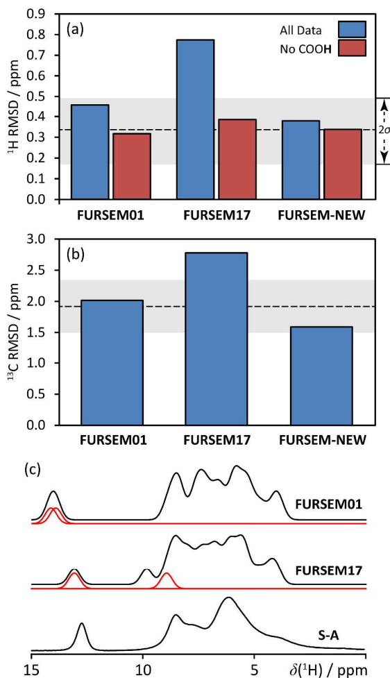
Fig. 3 Comparison of calculated and experimental \delta_{\text{iso}} of S-A and ReCryst with those computed using GIPAW DFT on the H-optimised structures indicated. Grey bands correspond to RMSD ranges established using a series of benchmark organics. § The ^1\text{H} RMSD is highly sensitive to the COOH hydrogen atom position, as shown by RMSD values which include (blue) and do not include (red) this site. (c) compares calculated ( FURSEM01 / FURSEM17 ) and experimental ( S-A ) ^1\text{H} NMR spectra. Red traces in (c) correspond to the carboxyl H atom from each crystallographically unique furosemide molecule.
