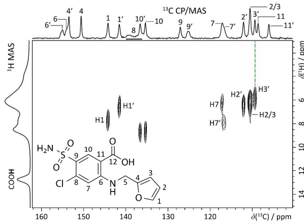
Fig. 2 Partial 1 H- 13 C refocused dipolar FSLG-HETCOR NMR spectrum ( B 0 = 11.7 T, T = 293(1) K; v MAS = 13.24 kHz, contact time = 100 μs) with site assignments for the furosemide molecule (inset, S-A sample). The top horizontal axis shows the 13 C CP/MAS NMR spectrum, while the left vertical axis corresponds to the 60 kHz 1 H MAS NMR spectrum of the same material. See ESI for a detailed account of the assignment.
