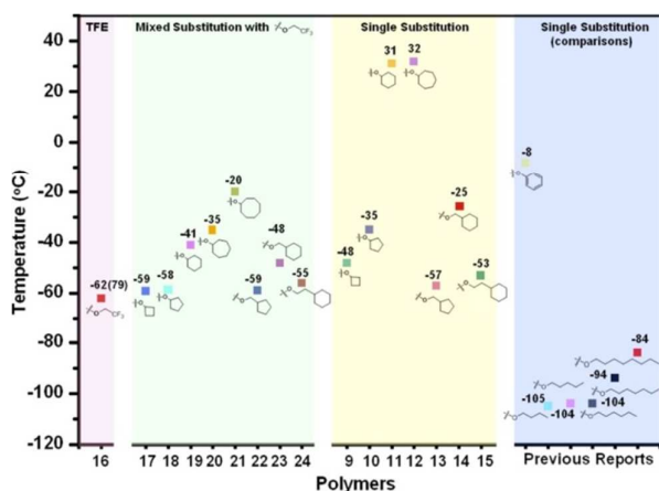
Fig. 2. The effect of different substituents on the glass transition temperatures of poly(organo)phosphazenes, exemplifying how small structural changes can be used to tailor the physical properties of the resulting polyphosphazene. Reprinted with permission from Z. Tian et al., Macromolecules , 2015, 48, 4301. Copyright 2015 American Chemical Society. 2
