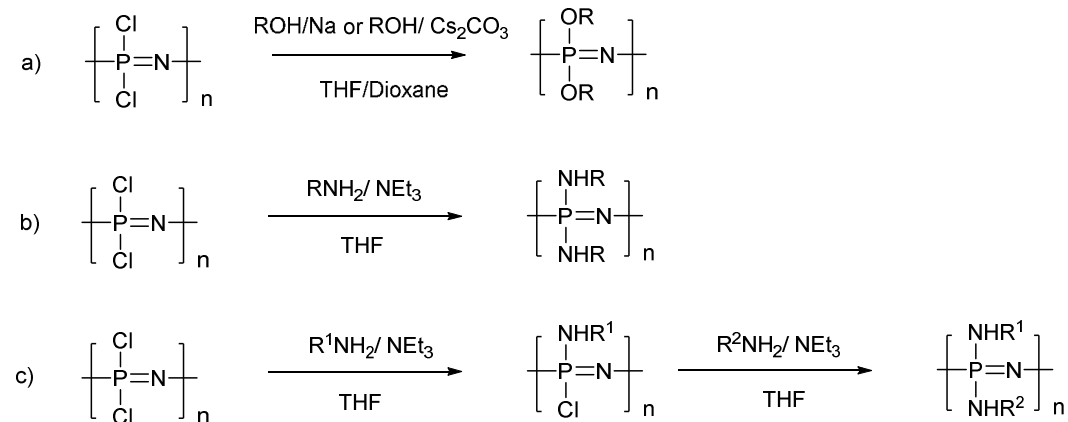
Fig. 3. The most common routes to poly(organo)phosphazenes via macromolecular substitution of the reactive precursor poly(dichloro)phosphazene using alkoxides or aryloxides (a) and primary amines (b). Scheme (c) depicts a mixed substitution using different nucleophiles which allows fine-tuning the properties of the polymer.
