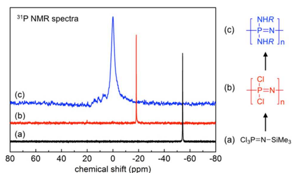
Fig. 4. Sample ^{31}\text{P}\{^1\text{H}\} NMR spectra of the monomer trichlorophosporanimine \text{Cl}_3\text{PNSiMe}_3 (a), polydichlorophosphazene [\text{NPCl}_2]_n (b) and a macrosubstituted poly(organo)phosphazene [\text{NP}(\text{NHR})_2]_n (c) demonstrating the simple tracking of the reaction progression. Adapted from H. Henke et al., J Polym Sci, Part A: Polym Chem , 2013, 51 , 4467. Copyright 2013 Wiley Periodicals, Inc. 12
