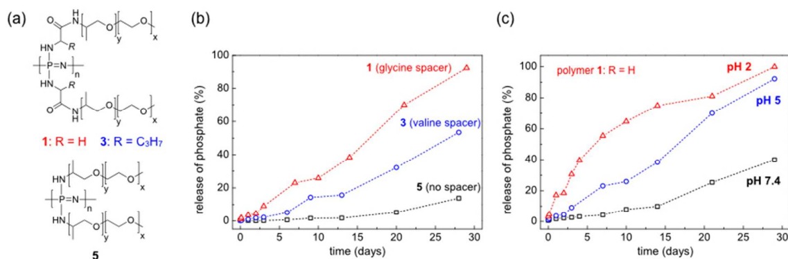
Fig. 27. Structures (a) and degradation profiles of some exemplary water-soluble, degradable poly(organo)phosphazenes, exemplifying the accelerating effect of hydrolysis by subtle changes in chemical structure (b) and at differing pH values (c). Relative degradation rates are measured by determination of the phosphate backbone degradation product. Adapted from S. Wilfert et al., J. Polym. Sci., Part A: Polym. Chem. , 2014, 52, 287. Copyright retained by authors. 49
