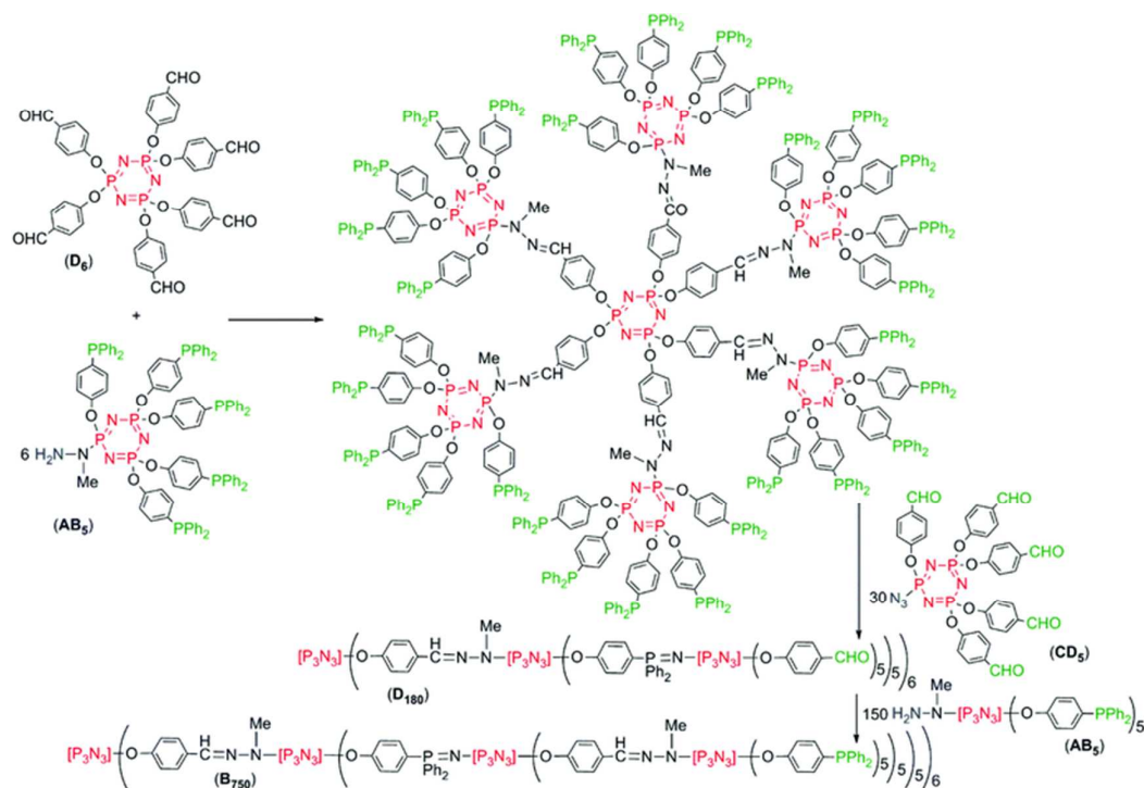
Fig. 20. An example of a highly branched dendrimer exploiting the cyclic phosphazene unit to insert a multiplying effect on the branching structure with an AB 5 type phosphazene based synthon on a hexachlorocyclotriphosphazene core. Reproduced from A.-M. Caminade, A. Hameau and J.-P. Majoral, Dalton Transactions , 2016, 45, 1810 with permission from The Royal Society of Chemistry. 40
