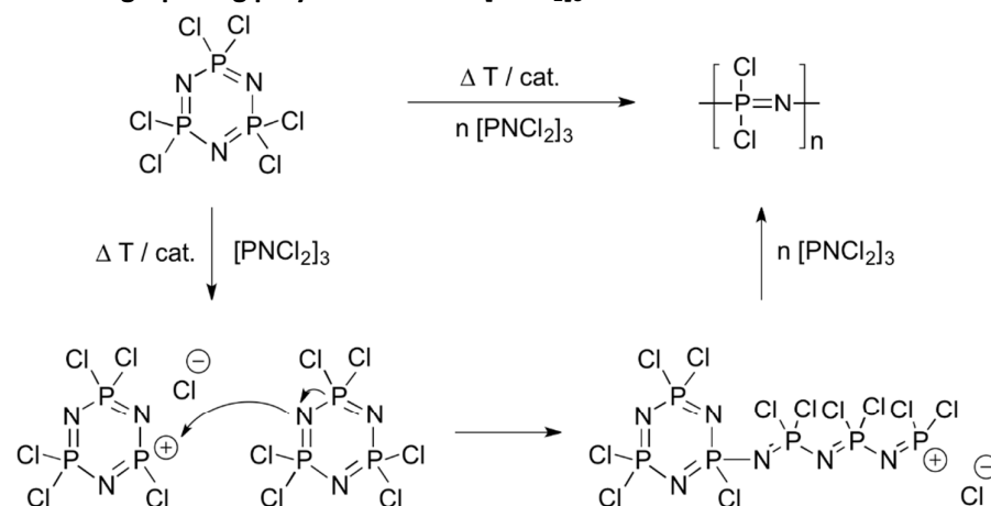
Fig. 5. Thermally and/or catalytically induced ring opening polymerisation representing the classical route to synthesise poly(dichloro)phosphazene [\text{NPCI}_2]_n and its commonly accepted mechanism.
