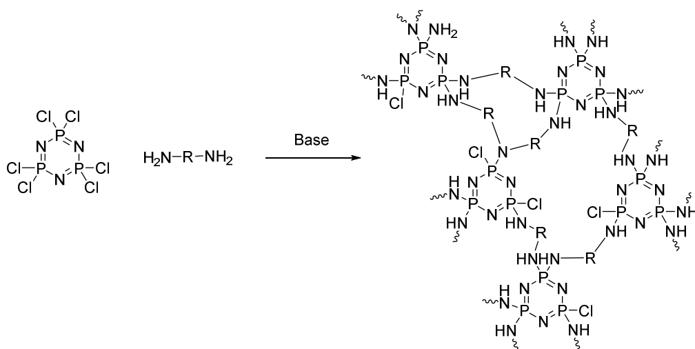
Fig. 18. An example synthesis route to cyclomatrix polyphosphazenes using hexachlorocyclotriphosphazene [NPCL 2 ] 3 as a building block.
