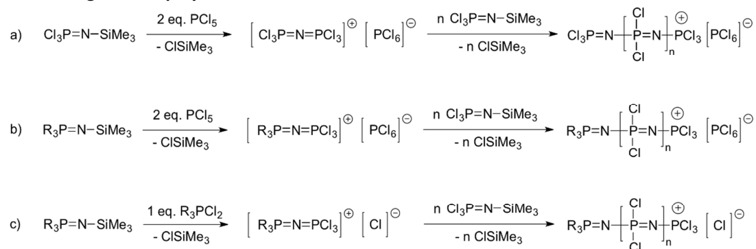
Fig. 6. Synthesis of poly(dichloro)phosphazene [\text{NPCl}_2]_n by living cationic polymerisation of trichlorophosphoranimine ( \text{Cl}_3\text{PNSiMe}_3 ) via initiation with \text{PCl}_5 (a), incorporation of alkyl or aryl substituted phosphoranimes for monodirectional growth (b) and phosphine-mediated polymerisation (c).
