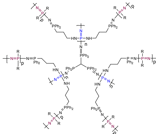
Fig. 12. Chemical structure of a polyphosphazene-based dendritic molecular brush, consisting of a star polyphosphazene (generation 1, 'n', shown in blue) which was used as a macroinitiator to grow polyphosphazene arms ('graft from', generation 2, 'p', shown in purple).
