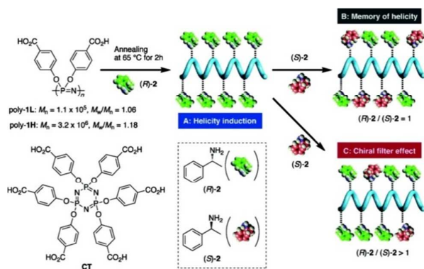
Fig. 17. Dynamic helicity of poly[di(4-carboxyphenoxy)phosphazene] and its application as a chirality filter. Note: The polymer referred to as Poly1L here is essentially PCPP, a well-known polyphosphazene investigated for use in medical applications. Reprinted with permission from K. Maeda et al., Macromolecules , 2011, 44, 2457. Copyright 2015 American Chemical Society. 36
