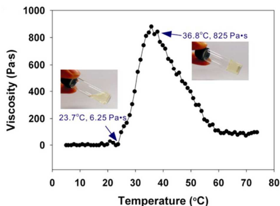
Fig. 24. Temperature-dependent sol–gel transition and viscosity change of a suitably functionalised poly(organo)phosphazene. Adapted with permission from Y.-M. Kim, M.-R. Park, and S.-C. Song, ACS Nano , 2012, 6, 5757. Copyright 2015 American Chemical Society. 46
