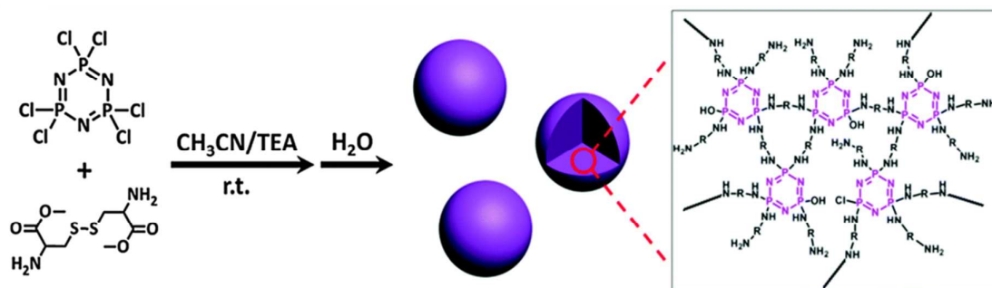
Fig. 19. An example of a precipitation condensation reaction to give cyclomatrix polyphosphazenes using [\text{PNCl}_2]_3 as a building block. Adapted from Z. Huang, S. Chen, X. Lu and Q. Lu, Chem. Commun. , 2015, 51, 8373 with permission from The Royal Society of Chemistry. 39
