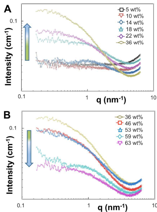
Figure 2: SAXS data recorded at 35 °C for THF-water mixtures without polymer from A) 5-36 wt% water and B) 36-63 wt% water.
