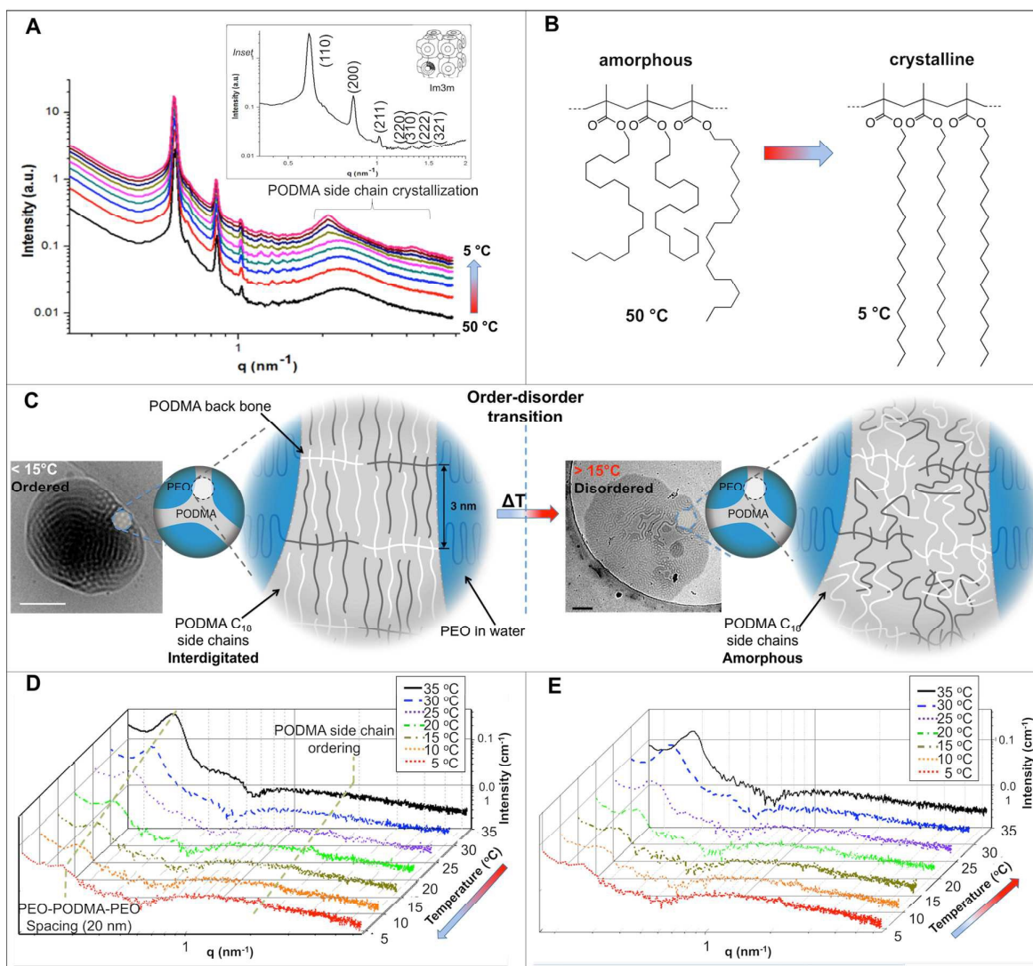
Figure 6: A) Temperature-resolved SAXS of the bulk material revealing the evolution of peaks corresponding to PODMA side chain crystallization between 2-5 \text{nm}^{-1} ; inset is an expansion of the q range 0-1.5 \text{nm}^{-1} , showing reflections of the Im3m phase in the bulk PEO- b -PODMA at 30 °C. B) representation of the change in the PODMA side chains at 50 and 5 °C. Temperature-resolved SAXS for the aqueous dispersion with C) decreasing temperature and D) increasing the temperature again. D) Schematic representation of the change in polymer molecule arrangement with temperature and the corresponding cryoTEM micrographs. Scale bars represent 200 nm.
