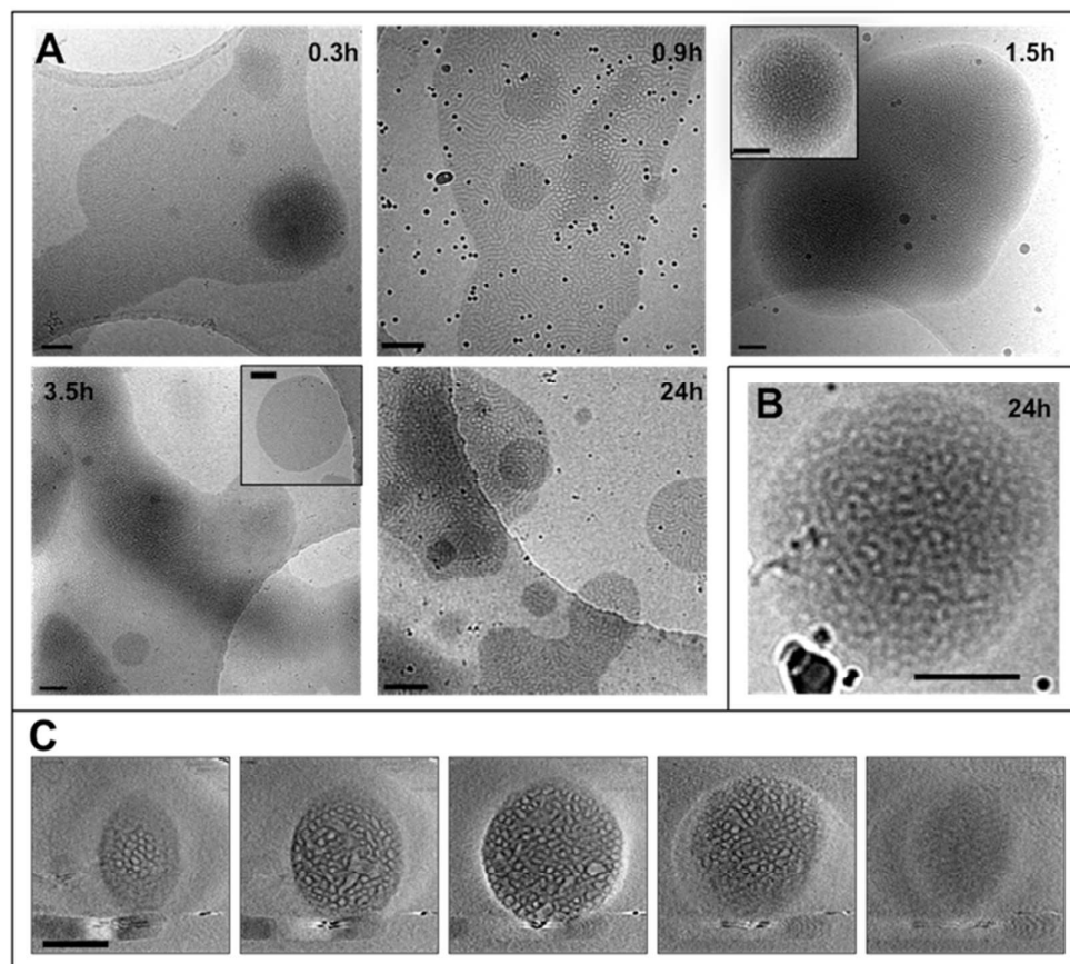
Figure 3: A) CryoTEM micrographs of the dispersions at different times during the dialysis period, black spheres are gold nanoparticles used as fiducial markers; B) cryoTEM image of a structured oblate spheroid from the dispersion at 24h; C) gallery of z-slices showing different cross sections of a 3D SIRT (simultaneous iterative reconstruction technique) reconstruction of a tomographic series recorded from the object shown in B. Scale bars represent 200 nm.
