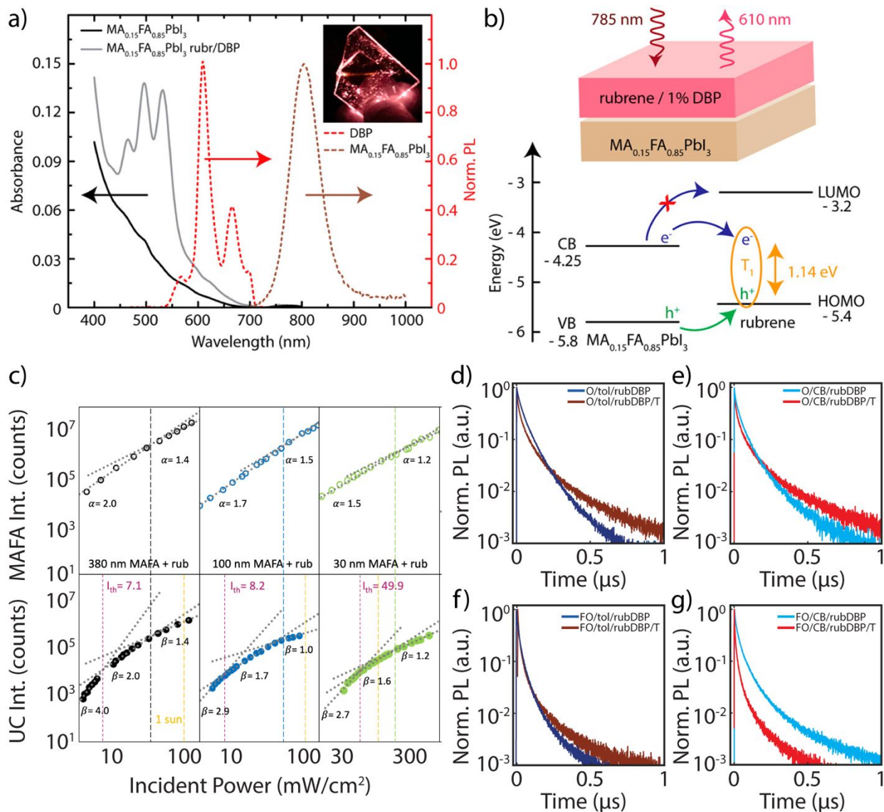
Figure 2: a) The absorbance (solid) and normalized PL emission (dashed) of the perovskite only (black) and perovskite/OSC device (gray). The UC emission stemming from the OSC layer (red) and PL emission from the perovskite (brown) are both highlighted. The inset shows the device under 785 nm illumination. b) A schematic of the device structure (top), where, upon 785 nm illumination, the OSC layer emits emission around 610 nm upon triplet sensitization via the perovskite layer. The rubrene triplet is occupied via sequential hole and electron transfer (bottom) from the perovskite valence and conduction band, respectively. Adapted with permission from Ref. [20]. Copyright 2019 American Chemical Society. c) Emission intensity of the perovskite emission (top 3 panels) and the UC emission (bottom three panels) at various fluences. Adapted from Ref. [21], Copyright 2019 Elsevier. d-g) PL emission decay of the perovskite emission of MA-rich films fabricated with overstoichiometric PbI 2 and either toluene (d) or chlorobenzene (e), and FA-rich films fabricated with overstoichiometric PbI 2 and either toluene (f) or chlorobenzene (g). Adapted with permission from Ref. [40]. Copyright 2020 John Wiley and Sons.
