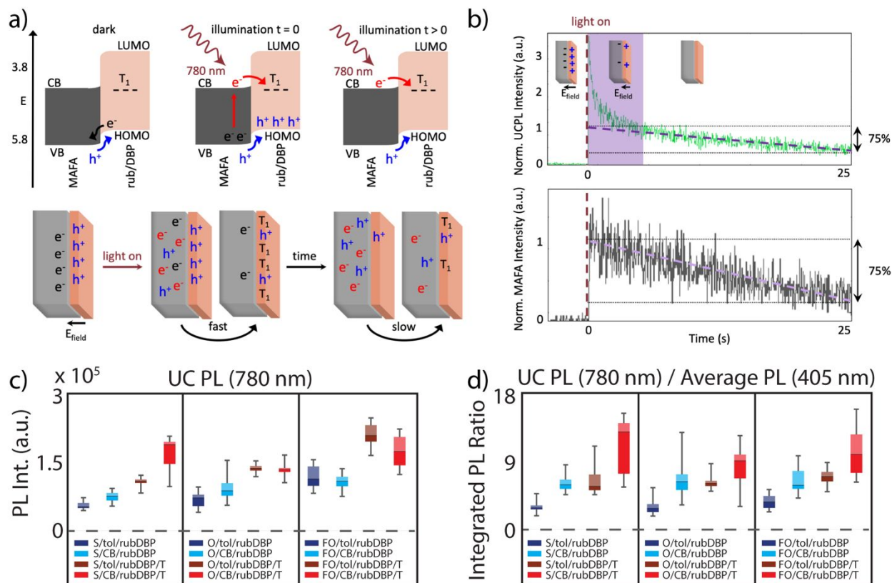
Figure 4: a) Top: band alignment of the perovskite (MAFA) and rubrene allow for hole transfer before illumination, resulting in a build-up of holes. Upon illumination, electron transfer occurs into the rubrene triplet state, and eventually, a steady-state occurs. Bottom: Schematic of the precharging effect described in a), where UC occurs much faster after illumination and then eventually slows down after rapid TTA at the interface. b) The UCPL (green) and perovskite emission (gray) over time, where the spike in the UCPL highlighted by the purple box occurs due to the build-up of charges at the interface, and then decreases. Adapted with permission from Ref. [45]. Copyright 2020 American Chemical Society. c) and d) Box plots detailing the UCPL intensity integrated from 500-700 nm (c) and the UCPL normalized by the PL under direct excitation at 405 nm for the various devices, where S, O, or FO denote stoichiometric PbI 2 MA-rich, overstoichiometric PbI 2 MA-rich, overstoichiometric PbI 2 FA-rich devices respectively. Additionally, either toluene or chlorobenzene is used to fabricate the OSC layer (denoted as tol or CB, respectively), and the films annealed post-fabrication are denoted with a T. Adapted with permission from Ref. [40]. Copyright 2020 John Wiley and Sons.
