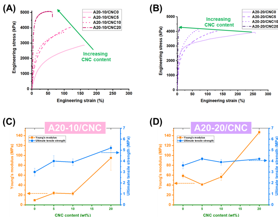
Figure 6. Representative stress-strain curves of (A) A20-10/CNC and (B) A20-20/CNC measured using a Zwick Roell mechanical testing machine (100 N load cell) in tension mode at room temperature under a constant strain rate of 100% of the initial gauge length/min. At least three samples with dimensions of \sim 3 \times 15 mm were tested for each material. Young's modulus ( E ) and ultimate tensile strength of (C) A20-10/CNC and (D) A20-20/CNC obtained by averaging the results of three samples, which highlight that the modulus is highly influenced by the PBLA content and CNC weight fraction compared with tensile strength. Young's modulus of A20-10/CNC nanocomposites increases from 9 MPa to 95 MPa with increasing CNC weight fractions from 0 wt% to 20 wt%, which contrasts with A20-20/CNC nanocomposites. Particularly, A20-20/CNC5 ( E = 41 MPa) exhibits a lower Young's modulus compared to neat A20-20 ( E = 59 MPa). Increasing the amount of CNCs in A20-20 to 20 wt% enables obtaining a higher Young's modulus up to 147 MPa. This tensile behavior reveals that a balance of peptidic ordering and PBLA-CNC interactions dictates the mechanical response of PPU/CNC nanocomposites.
