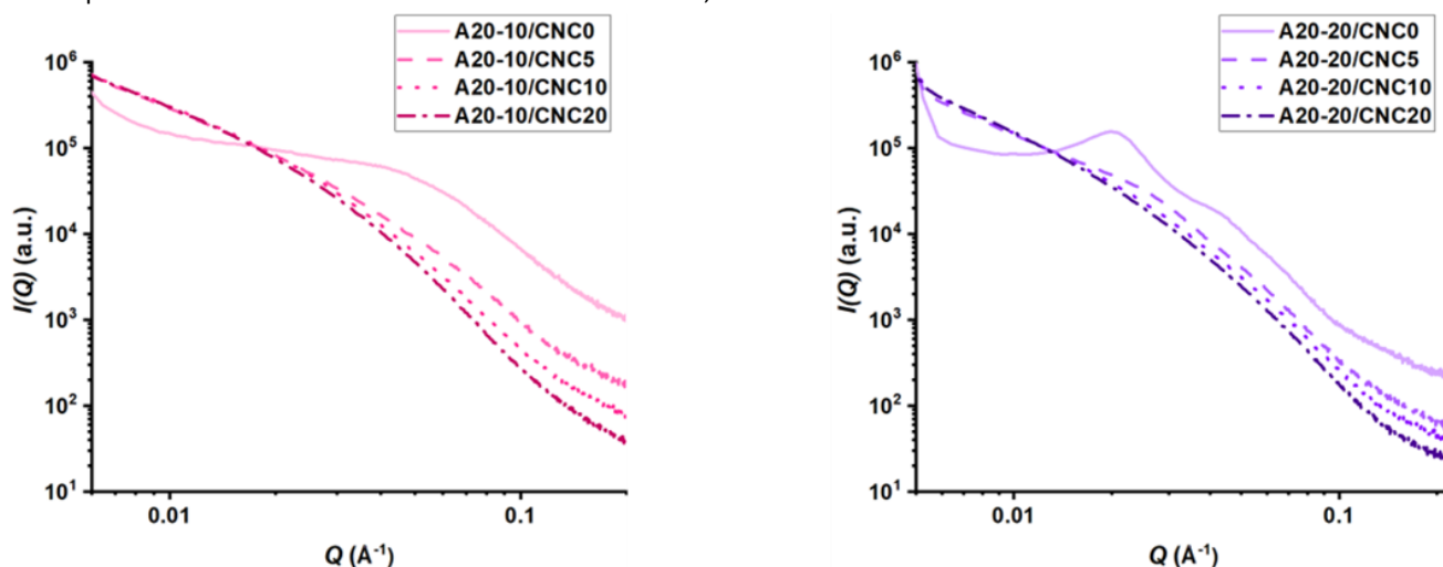
Figure 4. 1D-SAXS profiles of the PPU/CNC nanocomposites with varying PBLA and CNC content collected at room temperature for 30 minutes. The neat PPU matrices ( i.e. , A20-10/CNC0 and A20-20/CNC0) exhibit a defined scattering peak, whereas the addition of CNC to the matrices results in a reduction or loss of the distinct peak. These results indicate that the introduction of CNCs into PPU matrices modulates long-range ordering and structural hierarchy.
