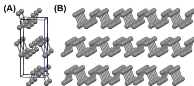
Fig. 1 The chemical structures of the compounds in this study. (A) The orthorhombic unit cell of black phosphorus 19 ( a = 3.31 Å, b = 4.38 Å, c = 10.50 Å, \alpha = \beta = \gamma = 90^\circ ; space group Bmab ; Crystallography Open Database ID: 1010325) which generates a layer structure comprising corrugated lamellae of phosphorus atoms held together by weak interlayer forces. (B) Three-layer phosphorene.
