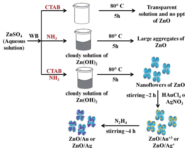
Scheme 1 The overall mechanism of ZnO/Au and ZnO/Ag nanoparticle formation on ZnO nanoflower surface. Here, WB represents water bath.
