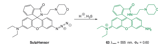
Fig. 60 Structure and reaction of Lyso-AFP .
