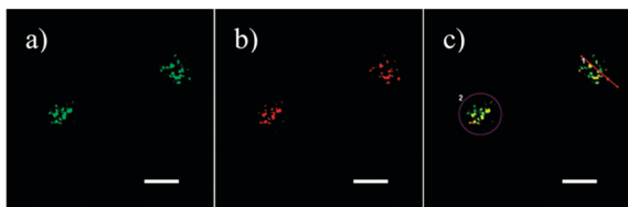
Fig. 61 Top: structure and reaction of SulpHensor . Bottom: HeLa cells stained with (a) LysoTracker Green (Ch1, green) and (b) SulpHensor (Ch2, red) with NaSH solution (c) overlay of (a) and (b). Scale = 10 \mu\text{m} . Image reproduced with permission. 233
