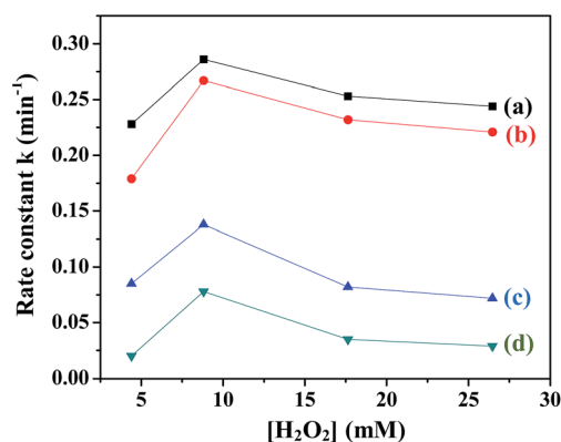
Fig. 9 Variation of rate constants with [H₂O₂] in the presence of (a) CuFe₂O₄, (b) ZnFe₂O₄, (c) NiFe₂O₄ and (d) CoFe₂O₄.
