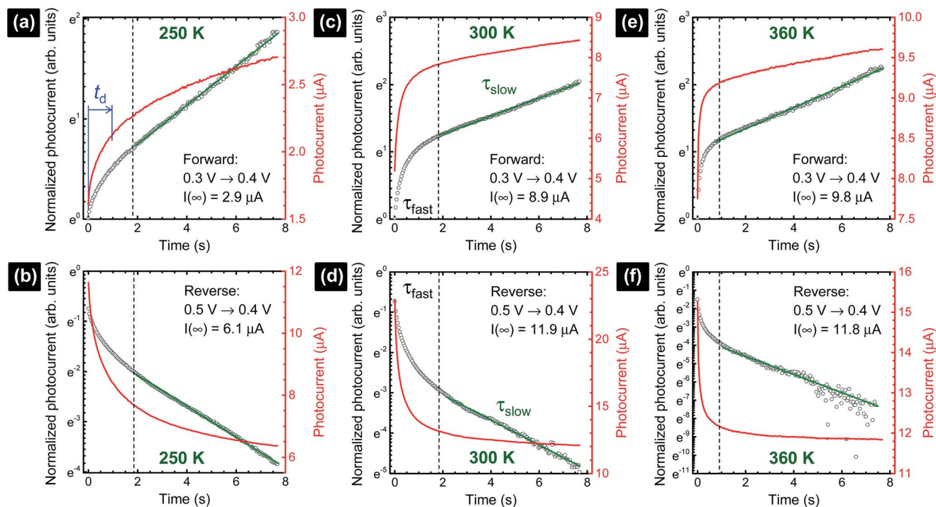
Fig. 3 Semi-logarithmic plot of the photocurrent responses as a function of time after applying a voltage step at t = 0 (a, c and e) from 0.3 \text{ V} \rightarrow 0.4 \text{ V} (forward) and (b, d and f) from 0.5 \text{ V} \rightarrow 0.4 \text{ V} (reverse) at (a and b) 250 K, (c and d) 300 K, and (e and f) 360 K. The spectra show that multiple processes, designated as \tau_{\text{fast}} and \tau_{\text{slow}} , take place during the charging–discharging within a perovskite solar cell. The degree of hysteresis depends on the waiting period to measure the photocurrent after applying a voltage, i.e., the delay time ( t_d ).
