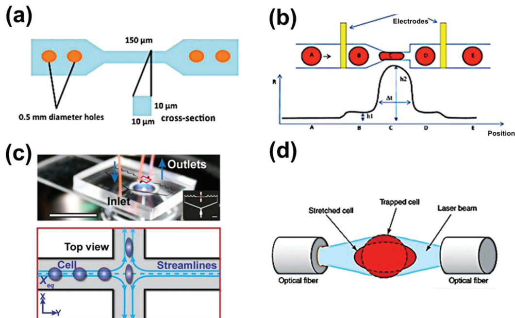
Fig. 2 Microfluidic technologies for measuring cell deformability. (a) Schematic representation of a straight channel microfluidic device with 150 μm length and 10 × 10 μm 2 cross-sectional area. The cell becomes deformed when it passes through the channel and different quantitative parameters, such as the entry time, transit velocity, and elongation index, were measured. Reproduced with permission from ref. 14. (b) Schematic representation of the suspended cells moving through the narrow constriction of a microfluidic device. As the cell moves, electrical resistance could be measured across the two electrodes placed on the either side of the constriction. This resistance increases from point A to a value 'h1' when the cell is positioned before point B. The resistance then peaks to a value 'h2' when the cell is constricted at point C and then drops again to 'h1' as the cell moves out at point D. Finally, the resistance returns to the baseline at point E when the cell crosses the downstream electrode. The time required by the cell to travel through the constriction is measured by the width of the signal (Δt). Reproduced with permission from ref. 17. (c) Top : photograph of a microfluidic device with inset showing the channel design developed for single-cell mechanophenotyping (the red region highlights deformation junction shown in the bottom figure). Bottom : cells are introduced into the microfluidic device and are stretched under continuous flow. The images of the stretched cells are captured using a complementary metal-oxide semiconductor (CMOS) camera. The cells are exposed to compressive and shear forces within the device, and the deformability and diameter of the cells are quantified to diagnose a cell as benign or malignant. Reproduced with permission from ref. 19. (d) Diagrammatic representation of the stretching of a cell in the axial direction using an optical stretcher. The optical forces from the two divergent laser beams trap the cell in the middle. When the laser power is increased, a force is generated on both the sides of the cell, thus stretching it along the laser beam axis. Reproduced with permission from ref. 20.
