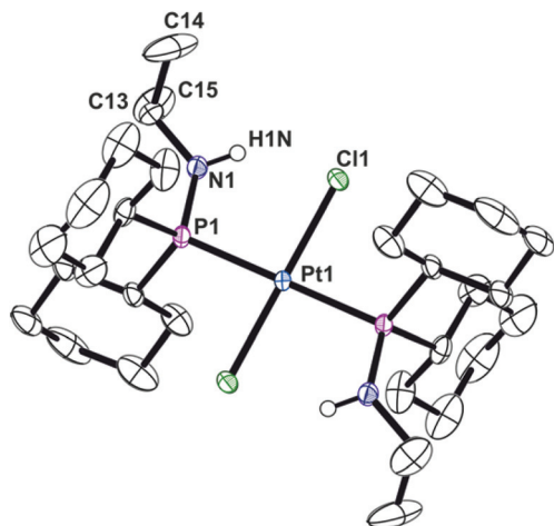
Fig. 3 Crystal structure of trans -[PtCl 2 (Cy 2 PNH t Pr) 2 ] ( 3 ). All hydrogen atoms have been omitted for clarity. Selected bond lengths (Å) and angles (°): Pt(1)–P(1) 2.3178(7), Pt(1)–Cl(1) 2.3193(7), P(1)–N(1) 1.681(3), Pt(1)–P(1)–N(1) 113.91(10).
