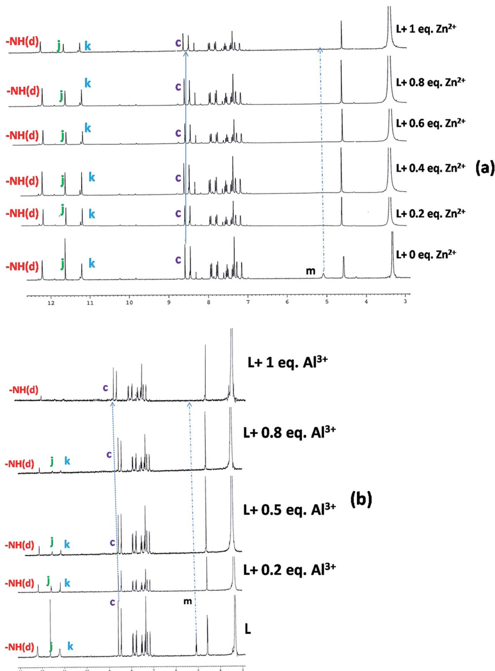
Fig. 6 ^1\text{H} -NMR titration of the free ligand (L = \text{H}_3\text{SAL-NH} ) and with the addition of 1 equivalent of \text{Zn}^{2+} (a) and \text{Al}^{3+} (b) in \text{DMSO}-d_6 recorded on a 300 MHz Bruker NMR spectrometer.
