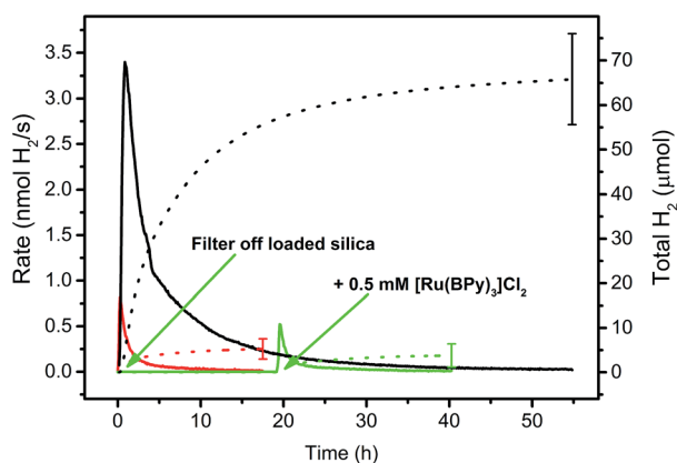
Fig. 2 Hydrogen evolution rate courses (solid lines) and total amounts of H_2 (dotted lines) in 1 M ascorbate buffer (pH 4) with 0.1 M NaOTf. Black: 20 \mu M 3 and 200 \mu M 5 adsorbed on hydrophobic fumed silica with 300 \mu M [C_{16}\text{-NMe}_3][\text{OAc}] (7) as surfactant. Green: same as black, but loaded silica was filtered off and the residual solution irradiated, then 0.5 mM [\text{Ru}(\text{bpy})_3]\text{Cl}_2 was added and irradiation continued (green arrows). Red: 0.5 mM [\text{Ru}(\text{bpy})_3]\text{Cl}_2 , no WRC. See Table S13.†
