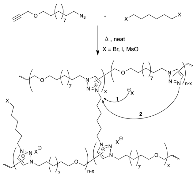
Fig. 6 Polymerisation of \alpha -azide- \omega -alkyne monomers with bifunctional alkylating agents results in polymer networks via the formation of 1,2,3-triazoles followed by the cross-linking process through alkylation to 1,2,3-triazoliums. The resulting networks can rearrange their topology through exchange between 1,2,3-triazoles and 1,2,3-triazoliums.
