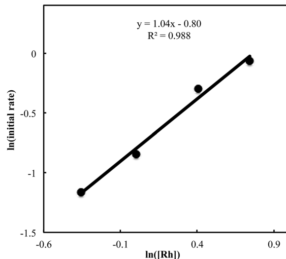
Fig. 4 \ln plot of the initial rate ( \text{mM min}^{-1} ) vs. concentration of Rh catalyst ( \text{mM} ) ( [\text{Rh}]_0 = 0.7\text{--}2.1 \text{ mM} , [\text{1a}]_0 = 50 \text{ mM} , [\text{2a}]_0 = 50 \text{ mM} ).
