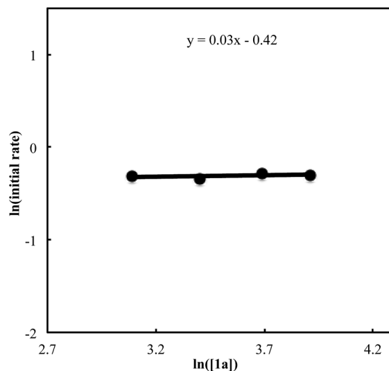
Fig. 5 \ln plot of the initial rate ( \text{mM min}^{-1} ) vs. concentration of triyne 1a ( \text{mM} ) ( [\text{Rh}]_0 = 1.5 \text{ mM} , [\text{1a}]_0 = 22\text{--}50 \text{ mM} , [\text{2a}]_0 = 50 \text{ mM} ).
