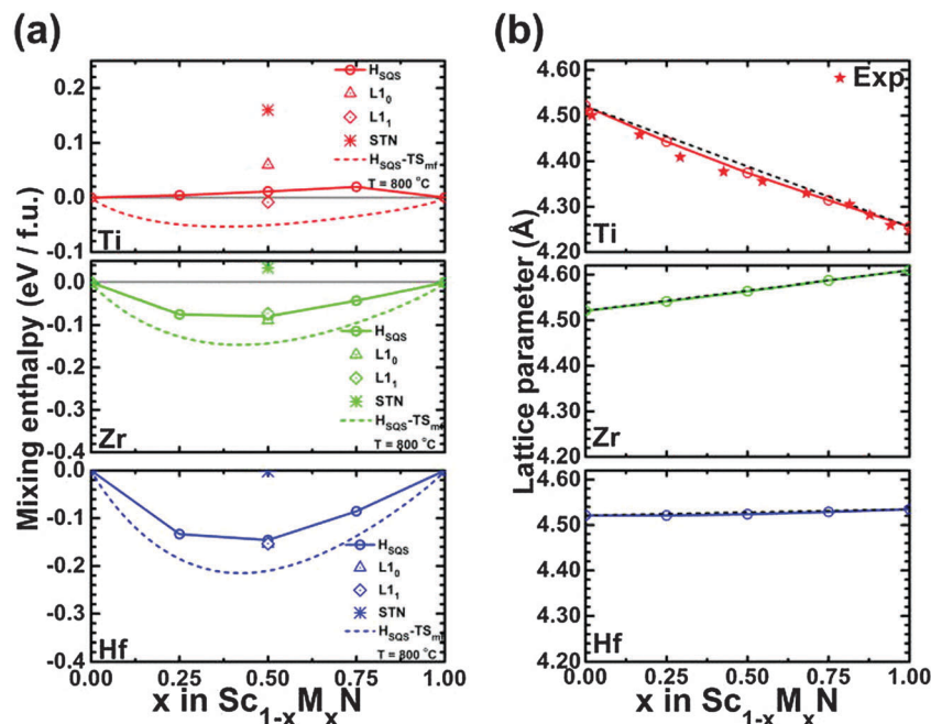
Fig. 5 (a) Comparison of the calculated mixing enthalpies of substitutionally disordered solid solution, ordered solid solutions and ScTa 2 -type structure phase of Sc 1-x M x N, as a function of MN content where M = Ti, Zr, and Hf, respectively. (b) Calculated equilibrium lattice parameter for rocksalt (B1) Sc 1-x M x N solid solution as a function of MN content where M = Ti, Zr, and Hf, respectively. The black line indicates Vegard's rule. For (Sc,Ti)N, experimental data from Gall et al. 22 are shown with stars. From ref. 96 (Copyright American Institute of Physics, used with permission).
