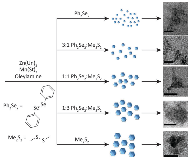
Fig. 1 General synthetic scheme for formation of \text{Mn}^{2+} -doped \text{ZnSe}_{1-x}\text{S}_x NCs. In the reaction, zinc undecylenate, \text{Zn}(\text{Undecylenate})_2 , manganese stearate, \text{Mn}(\text{Stearate})_2 , and a mixture of diphenyl diselenide and dimethyl disulphide (or diphenyl disulphide) are combined and heated to reaction temperature in an alkylamine under an inert atmosphere. Depending on the ratio of diselenide to disulphide, NCs of different shapes and sizes are obtained. Images of samples 1–5 are shown. Scale bars are 20 nm.
