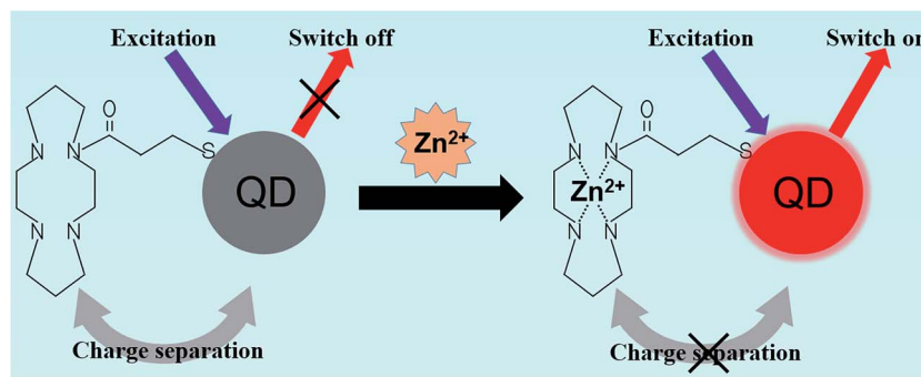
Fig. 6 Schematic principle of zinc ion nanosensors. Conjugation of QDs and azamacrocycles causes charge separation and quenching of QDs. The complexation of \text{Zn(II)} with the ligand changes the energy level on the ligand, which prevents the charge separation and leads to the fluorescence recovery of QDs. Reproduced from ref. 106 with permission. Copyright © 2008, American Chemical Society.
