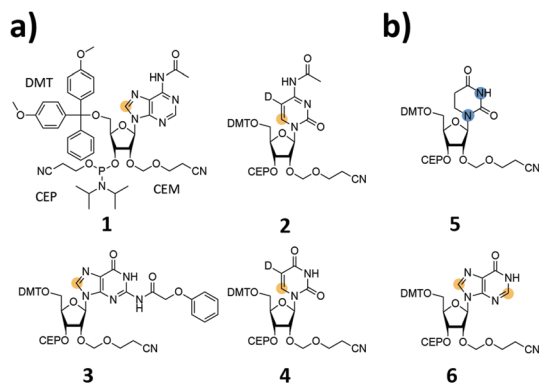
Fig. 1 Stable isotope (SI) labelled 2'-CEM RNA phosphoramidites. (a) 8- ^{13}\text{C} -purine (1 A; 3 G) and 6- ^{13}\text{C} -pyrimidine (2 C; 4 U) labelled 2'-CEM RNA phosphoramidites. (b) Naturally occurring SI-labelled building blocks: the 1,3- ^{15}\text{N}_2 -dihydrouridine 2'-CEM (5) and the 2,8- ^{13}\text{C}_2 -inosine 2'-CEM RNA phosphoramidites (6). Both modifiers are frequently found in transfer RNAs. Orange dot = ^{13}\text{C} , blue dot = ^{15}\text{N} .
