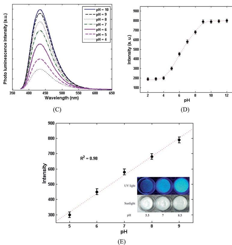
Fig. 6 (A) The alteration of pH for acute and chronic wounds. (B) Visual images for illustration of the pH sensitivity of CDs at different pH under UV 365 nm (top) and daylight (down). (C) The fluorescence spectra of CDs at various pH values and 365 nm excitation. (D) Variation of the fluorescence intensities of CDs at different pH values. (E) The linearization of the fluorescence intensity and pH values for 1.0 wt% chitosan/CDs nanocomposite. Inset: photograph of the fluorescence composite at various pH values under UV and daylight.
