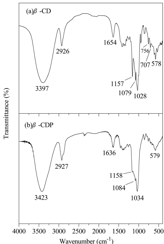
Fig. 5 FTIR spectra of β-CD (a) and β-CDP (b).
