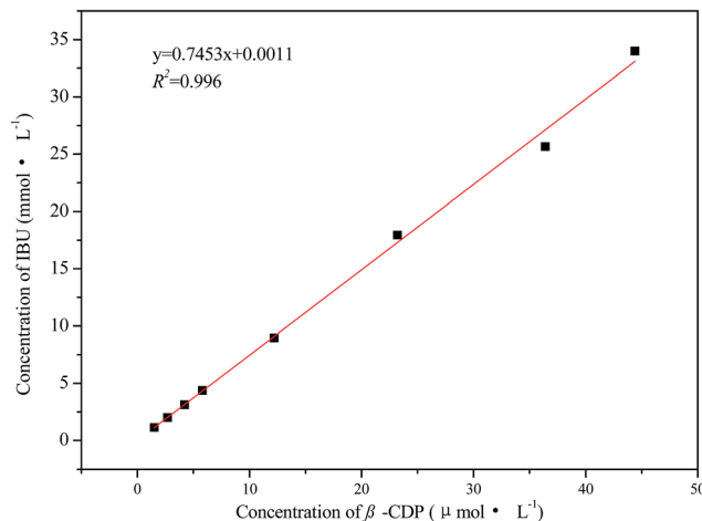
Fig. 6 Phase-solubility diagram of IBU in aqueous solutions of β-CDP.
