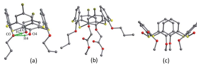
Fig. 36 Crystal structures of 44 (a), 45 (b) and 46 (c).
