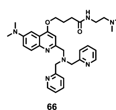
Scheme 52 Fluorescent probe 66 for Zn 2+ .
