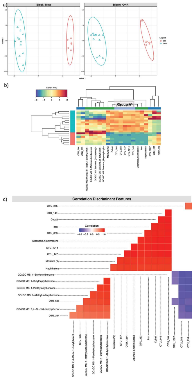
Fig. 6 DIABLO 2. (a) The algorithm found two components reducing the classification error rates in the DIABLO algorithm and shows the ordination of samples with ellipses representing 95% confidence interval and percentage variations explained by these components in axes labels for both microbiome (Block: rDNA) and meta data (Block: Meta). (b) shows the heatmaps of these discriminant features, with both rows and columns ordered using hierarchical (average linkage) clustering to identify blocks of features of interest. Group A' (Table 2) is indicated in a grey box. (c) shows the significant correlations ( -0.6 < R > 0.6 ) between the features as calculated by the algorithm.
