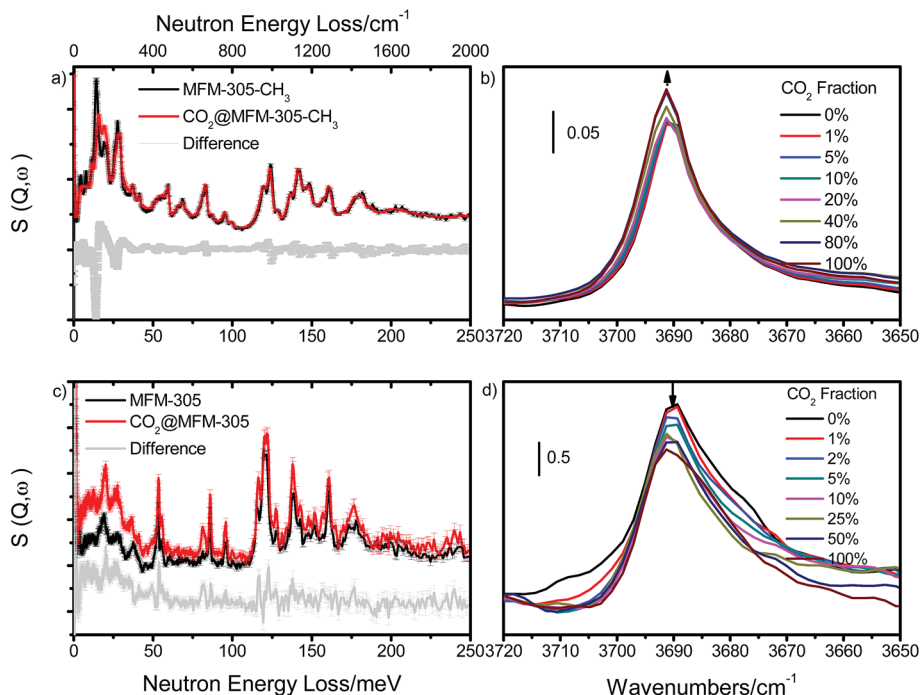
Fig. 5 Comparison of (a and c) the INS spectra and (b and d) IR spectra for bare MFM-305-CH 3 and MFM-305. INS and IR spectra offer vibrational information on the -\text{CH}_3/-\text{CH}/-\text{OH} stretching and deformation region. (a) Comparison of the INS spectra for bare and CO 2 -loaded MFM-305-CH 3 . (b) IR spectra in the \nu(\mu_2\text{-OH}) stretch region of CO 2 -loaded MFM-305-CH 3 . (c) Comparison of the INS spectra for bare and CO 2 -loaded MFM-305. (d) IR spectra of the \nu(\mu_2\text{-OH}) stretch region of MFM-305 for CO 2 -loading. IR and INS data were collected at 298 K and 5 K, respectively.
