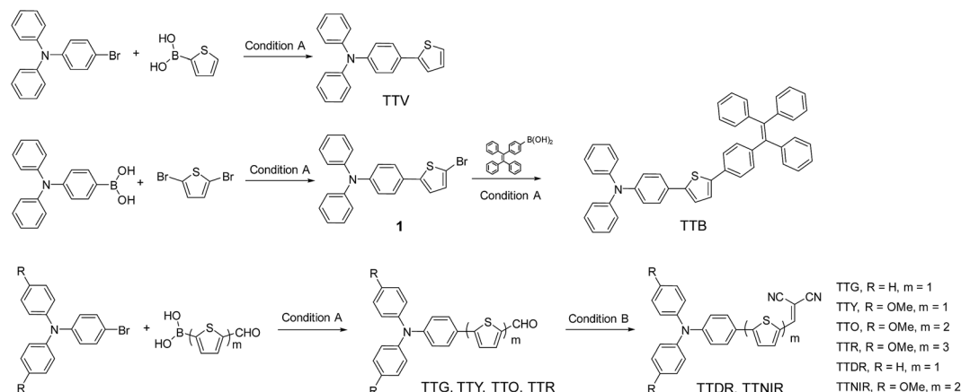
Scheme 1 Synthetic routes to AIEgens with tunable emission colors. Condition A: \text{Pd}(\text{PPh}_3)_4 , \text{K}_2\text{CO}_3 , THF, \text{H}_2\text{O} , 75^\circ\text{C} , 12 h. Condition B: EtOH, malononitrile, 78^\circ\text{C} , 72 h.
