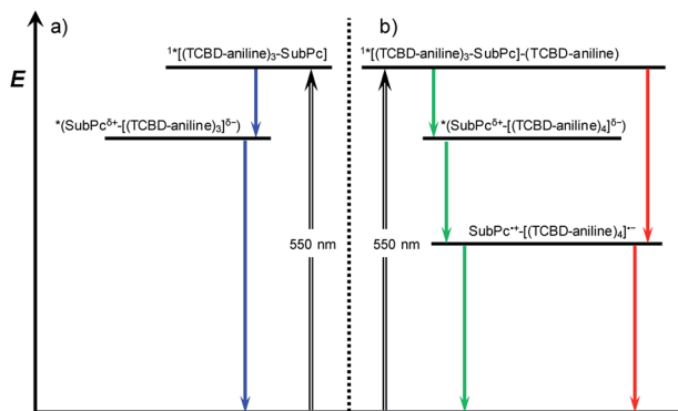
Fig. 5 Energy level diagram of (a) (TCBD-aniline) 3 -SubPc(4BuPhO) 1 in toluene, chlorobenzene, anisole, and benzonitrile (blue arrows) and (b) (TCBD-aniline) 3 -SubPc(TCBD-aniline) 2 in chlorobenzene and anisole (green arrows), and benzonitrile (red arrows) reflecting the energetic pathways after excitation of SubPc ( \lambda_{\text{ex}} = 550 nm, black arrow). Blue, green, and red arrows refer to nonradiative processes.
