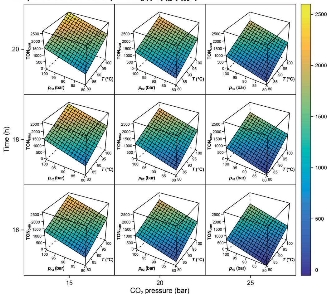
Fig. 3 Calculated response surfaces. (A) Trellis plot of the response surface for g_3(n_{\text{cat}}, n_{\text{add}}, V) from OLS modelling with T = 90\text{ }^\circ\text{C} , p_{\text{H}_2} = 90\text{ bar} , p_{\text{CO}_2} = 20\text{ bar} and t = 18\text{ h} . (B) Response surface trellis plot of the linear OLS model for g_1(T, p_{\text{H}_2}, p_{\text{CO}_2}, t) with n_{\text{cat}}^* = 0.075\text{ }\mu\text{mol} , n_{\text{add}}^* = 3.576\text{ }\mu\text{mol} and V^* = 0.550\text{ mL} . For a mathematical definition of the polynomial parametric surrogates, g_{1,3}() , see the Methods section.
