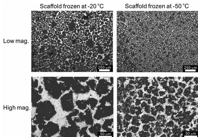
Fig. 4 SEM top views of the sintered LLZO scaffolds, frozen at -20^{\circ}\text{C} and -50^{\circ}\text{C} , respectively, at low and high magnifications.
