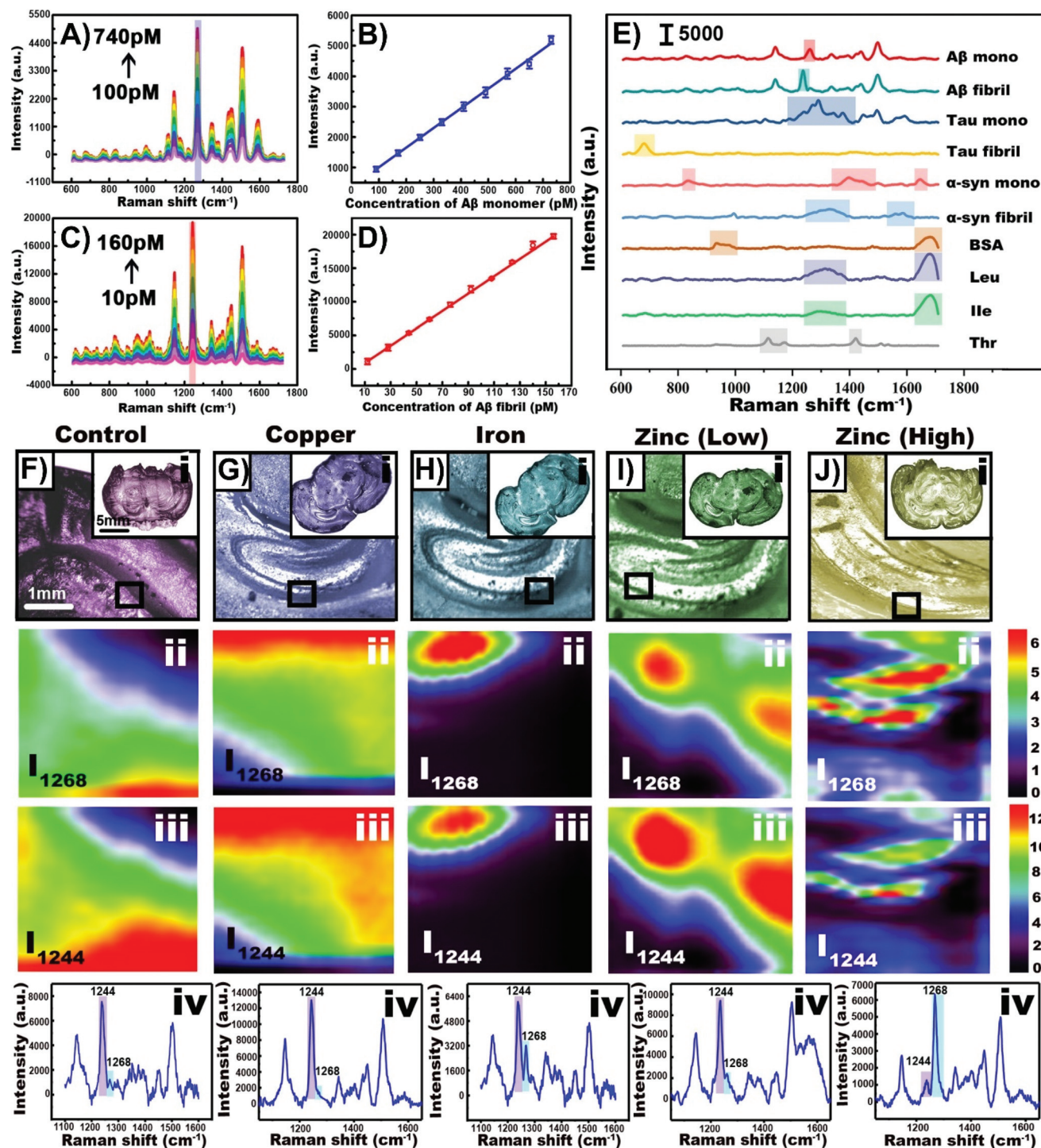
Fig. 8 (A) SERS spectra of gold nanoparticles synthesized with A\beta_{40} monomer with concentrations ranging from 100 to 740 pM. (B) Plot of SERS intensity at 1268 cm^{-1} with varying monomer concentration. (C) SERS spectra of gold nanowalnuts synthesized with A\beta_{40} fibril with concentrations ranging from 10 to 160 pM. (D) Plot of SERS intensity at 1244 cm^{-1} with varying fibril concentration. (E) SERS spectra obtained using various bio-molecules and the template method. (F–J) Results obtained for mice given different diets. (i) Bright-field images of tissue slices obtained from the treated transgenic mice. SERS imaging of A\beta_{40} in the hippocampus in the tissue slices at (ii) 1268 cm^{-1} and (iii) 1244 cm^{-1} . (iv) SERS spectra of A\beta_{40} in the hippocampus. Adapted with permission from Anal. Chem. , 2020, 92, 5910–5920 (ref. 122). Copyright (2020) American Chemical Society.
