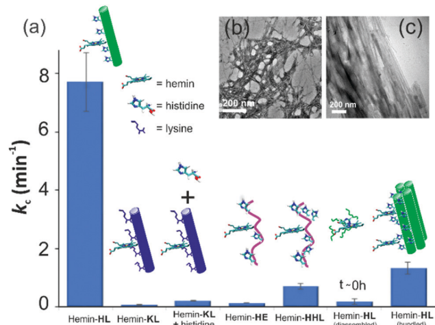
Fig. 3 (a) Tandem activity with MPA. TEM images of (b) HE nanofibers and (c) bundled HL. [Hemin] = 0.01 mM, [peptide] = 1 mM, [ \text{H}_2\text{O}_2 ] = 30 mM, [MPA] = 5 to 30 mM. Results are reported in triplicates.
