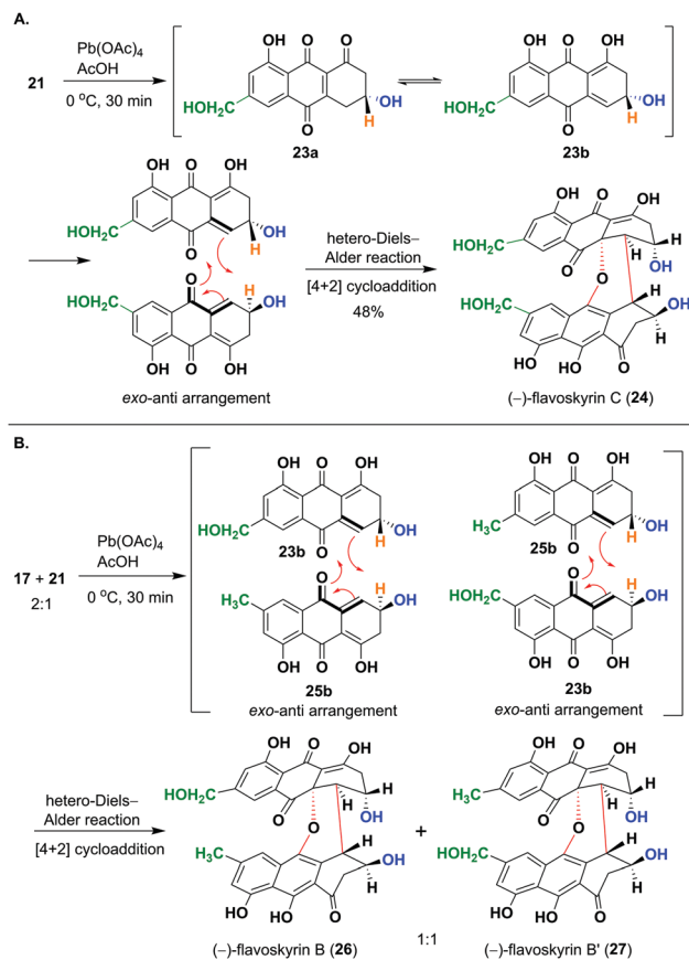
Scheme 3 (A) Oxidation of 21 by Pb(OAc) 4 forms (–)-flavoskyrin C ( 24 ) through the hetero Diels–Alder reaction. (B) Oxidation of a mixture of 17 and 21 (2 : 1) by Pb(OAc) 4 yielded flavoskyrin B ( 26 ) and flavoskyrin B' ( 27 ) as a major product.
