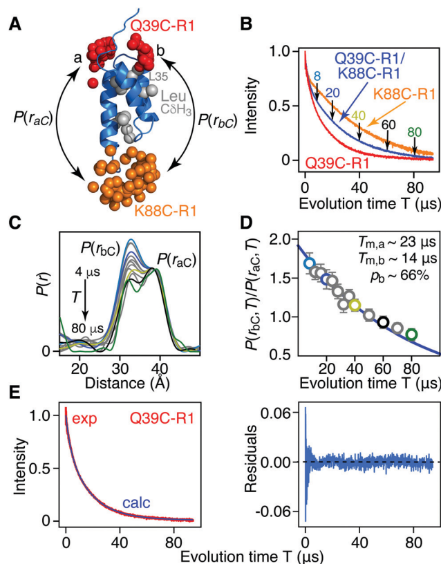
Fig. 2 Phase memory relation time ( T_{\text{m}} ) filtering for [ \text{Leu-CH}_3/2\text{H} ]AviTag-Protein A (Q39C-R1/K88C-R1) in an otherwise perdeuterated background. (A) Ribbon diagram of the protein A core domain 22 (blue) with the oxygen atoms of the nitroxide spin label ensembles (generated using the rotamer library program MMM) colored in red (Q39C-R1) and orange (K88C-R1), and the leucine methyl groups in grey. The two distances between K88C-R1 and the two conformer populations ( a and b ) of Q39C-R1 are indicated. (B) Hahn spin-echo curves for [Leu-CH 3 /2H]AviTag-Protein A, spin-labeled at Q39C-R1/K88C-R1 (blue), Q39C-R1 (red) and K88C-R1 (orange). (C) P(r) distributions for [Leu-CH 3 /2H]AviTag-Protein A (Q39C-R1/K88C-R1) obtained from the DEER echo curves using DeerAnalysis 24 with Tikhonov regularization at evolution times T ( = 2\tau_2 ) ranging from 8 to 80 \mu s. The color coding corresponds to that of the experimental points in panel D. The P(r) distributions are normalized with regard to the peak at 38 Å. The DEER pulse scheme is shown in Fig. S1B (ESI†), and the raw and background-corrected DEER echo curves are shown in Fig. S3 (ESI†). Results of global best-fitting eqn (1) and (2) to the experimental evolution time T ( = 2\tau_2 ) dependence of (D) the peak intensity ratio, P(r_{\text{bC}}, T)/P(r_{\text{aC}}, T) , in the P(r) distributions for [Leu-CH 3 /2H]AviTag-Protein A (Q39C-R1/K88C-R1) and (E) the Hahn echo curve for [Leu-CH 3 /2H]AviTag-Protein A (Q39C-R1) (left panel). The experimental ratios of the b to a peak intensities, P(r_{\text{bC}}, T)/P(r_{\text{aC}}, T) , are obtained from the integrated intensities of two Gaussians fitted to the bimodal P(r) distributions. The experimental data and best-fits are displayed by the circles and blue line, respectively in (D) and by the red and blue curves, respectively, in (E). Normalization in (E) was carried out by dividing the experimental and calculated curves by the optimized value of the sum of the two scale factors ( \lambda_1 + \lambda_2 ). The right panel in (E) is a plot of the distribution of residuals between experimental and calculated Hahn echo curves. The corresponding P(r) distributions and best fits obtained using DeerAnalysis with validated Tikhonov regularization, 24 the program DD with a sum of two Gaussians, 25 the program WavPDS (to filter out noise) 26 followed by Tikhonov regularization, 24 and WavPDS followed by SVD 26–28 are shown in Fig. S4–S7 (ESI†), respectively.
