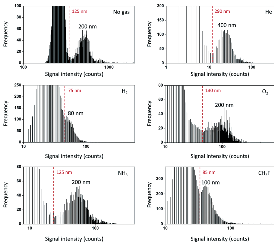
Fig. 4 Frequency distribution for the lowest NP sizes detectable using different reaction gases in ICP-TQ-MS for \text{SiO}_2 particle analysis. Practical \text{LOD}_{\text{size}} are indicated in red in each figure. Frequency refers to the number of events of each type (background or NPs) detected. Reproduced from Bolea-Fernandez et al. 56 with permission from the Royal Society of Chemistry.
