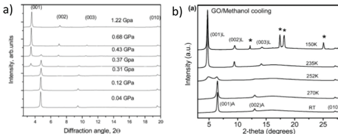
Fig. 10 Pressure (a) and temperature (b) induced phase transition from the ambient 1-layer Brodie GO–methanol structure to a 2-layer structure. (a) XRD patterns ( \lambda = 0.7092 \text{ Å} ) recorded from Brodie GO immersed in excess of liquid methanol upon pressure increase. 112 (b) XRD patterns recorded in the process of cooling ( \lambda = 0.99874 \text{ Å} ). 209
