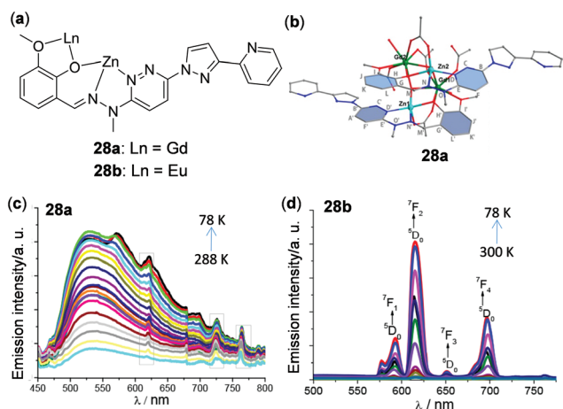
Fig. 24 (a) Structure segment of the \text{Zn}_2\text{Ln}_2 clusters 28a and 28b . (b) Cation core structure of 28a . (c and d) Temperature-dependent emission spectra of (c) 28a ( 78\text{--}288\text{ K} ) and (d) 28b ( 78\text{--}300\text{ K} ) with excitation at 350\text{ nm} . The three sharp peaks marked with a gray rectangle in panel (c) are the emission spectra of a background light source. Reprinted with permission from ref. 125. Copyright 2017 American Chemical Society.
