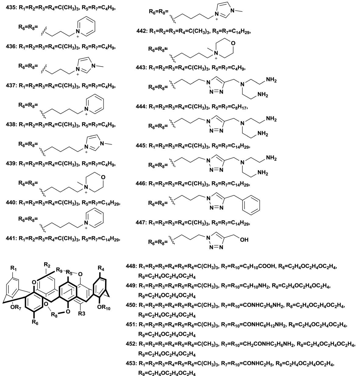
Scheme 4 Structures of bola-type amphiphilic calixarenes.
