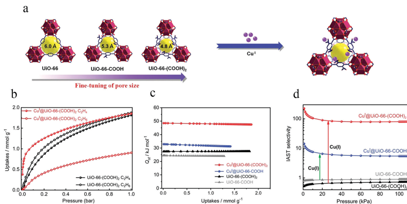
Fig. 4 (a) Single-crystal X-ray structures of UiO-66-type MOFs. (b) Single-component adsorption isotherms for C_2H_4 and C_2H_6 on UiO-66-(COOH) 2 and Cu@UiO-66-(COOH) 2 at 298 K. (c) Isostatic heat ( Q_{st} ) of C_2H_4 adsorption on the UiO-66-type MOFs. (d) IAST calculations of activated UiO-66-type MOFs for C_2H_4/C_2H_6 separation at 298 K.
