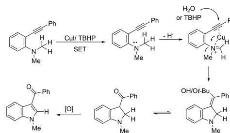
Scheme 34
