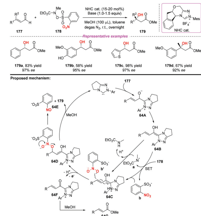
Scheme 64 Chiral NHC-catalyzed \beta -hydroxylation of enals using nitroarenes as an oxidant.
