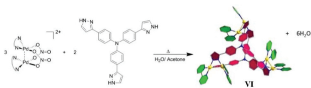
Fig. 18 Representation of self-assembly of cage VI , [M_6L_2] using dimeric corners. Reproduced with permission from ref. 79. Copyright 2017, Royal Society of Chemistry.
