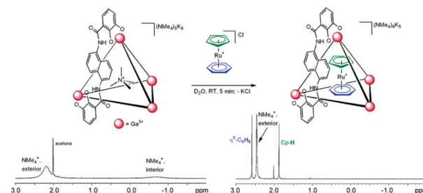
Fig. 4 NMe_4^+ guest exchange with 2, K_6(NMe_4)_5[II^e_{Ga}NMe_4] before (left), and after (right) the addition of [CpRu(\eta^6-C_6H_6)]^+ . Reproduced with permission from ref. 47. Copyright 2004, American Chemical Society.
