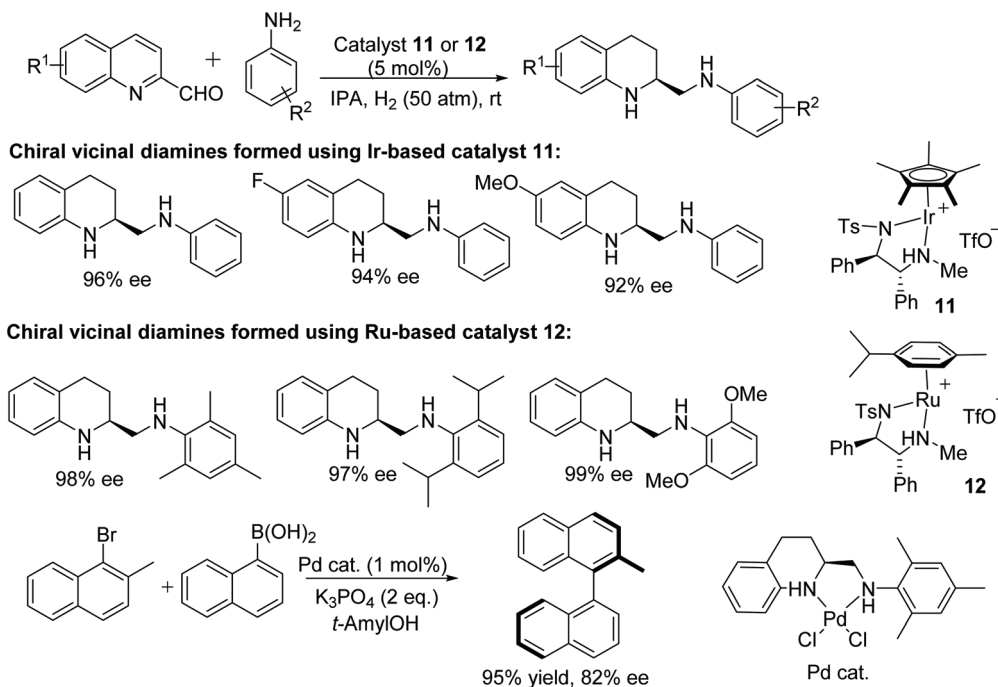
Fig. 17 Synthesis of chiral N,N' -diaryl vicinal diamines by AH and application of the diamine product in Suzuki coupling.
