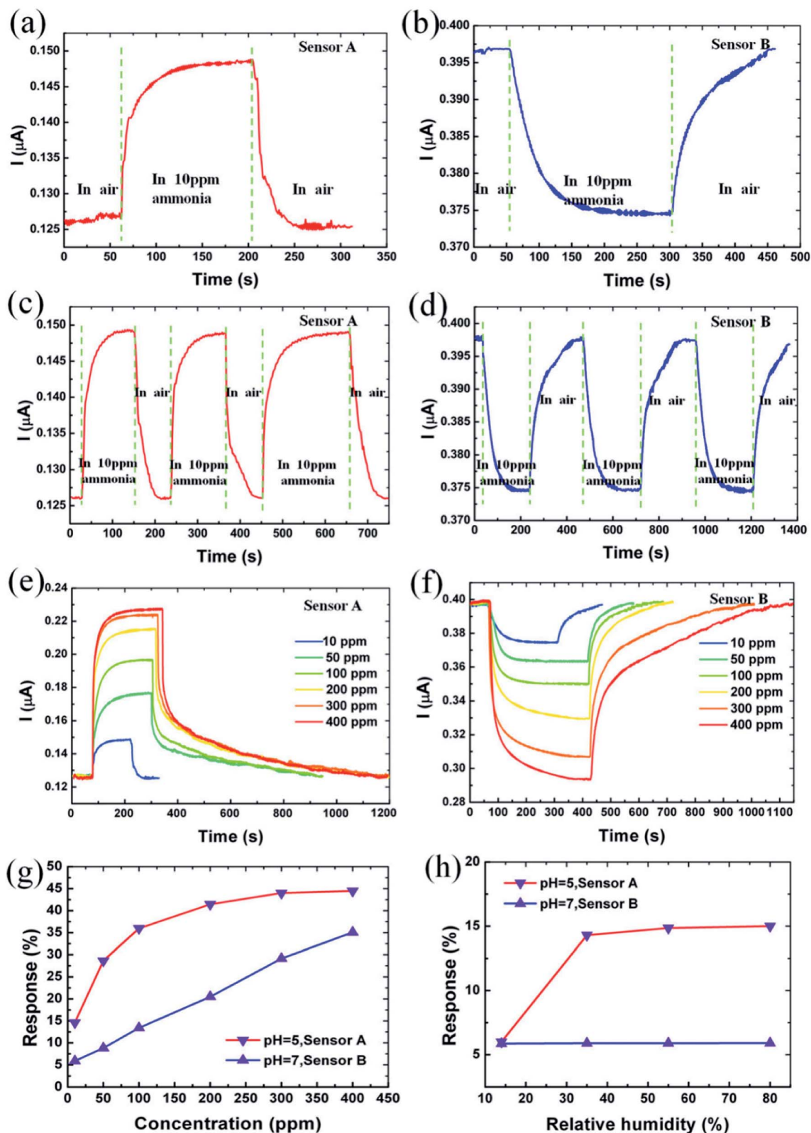
Fig. 15 (a and b) 10 ppm ammonia response characteristic of sensor A and B, respectively. (c and d) Response of sensor A and B to 10 ppm NH 3 for three cycles, respectively. (e and f) Current response behaviour for sensor A and B at different concentrations of NH 3 ambient (g) absolute response of sensors A and B at various concentrations of NH 3 (h) absolute response of sensors A and B to 10 ppm NH 3 at various relative humidity. Reproduced with permission from ref. 150, copyright 2016, Elsevier.
