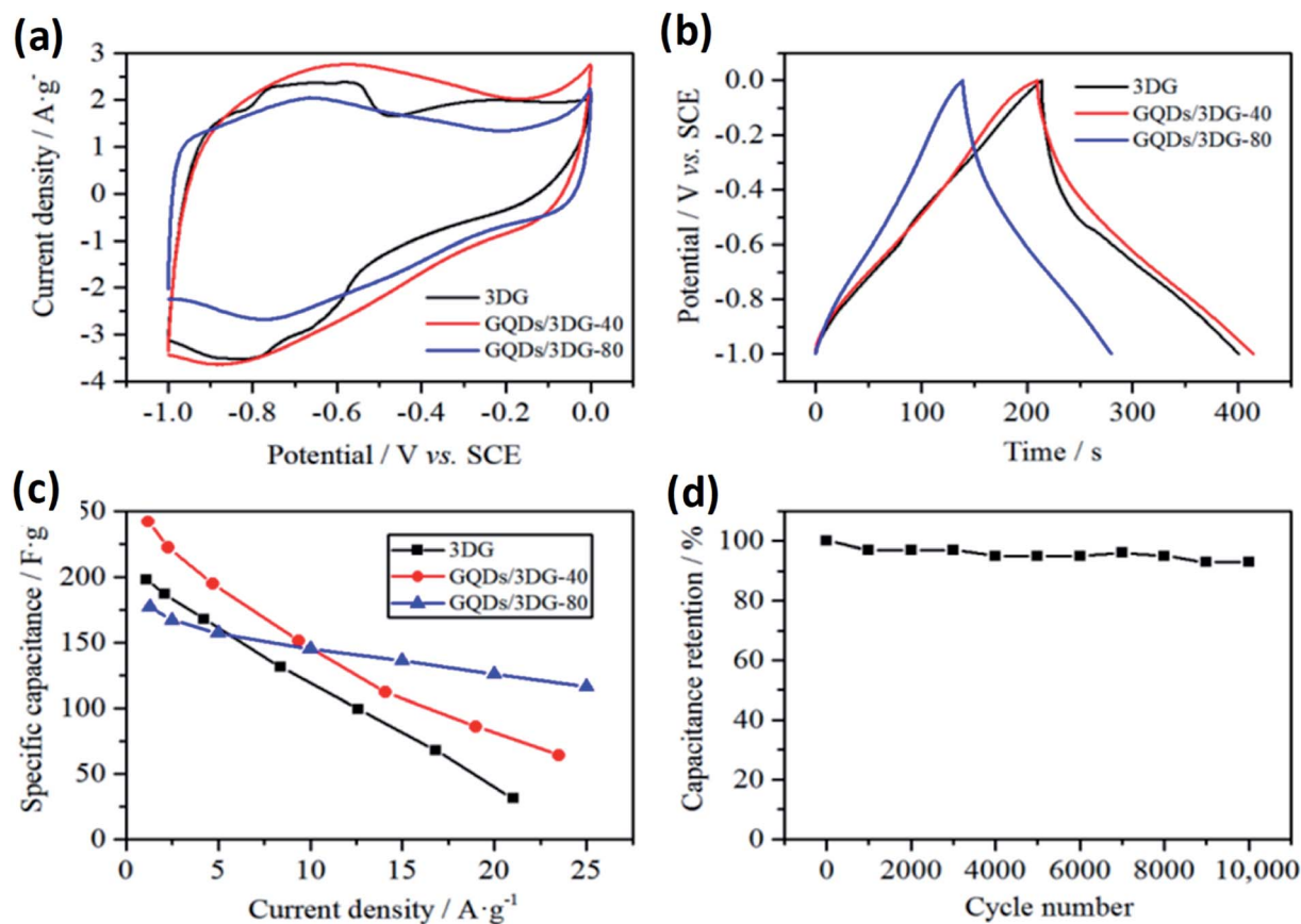
Fig. 18 (a) Cyclic voltammogram curve at a scan rate of 10 \text{ mV s}^{-1} (b) charge/discharge curves at different current densities with different compositions, respectively (c) specific capacitance versus current densities and (d) cycling stability at a current density of 24 \text{ A g}^{-1} for the composite material. Adapted from ref. 183, copyright 2019, MDPI publications.
