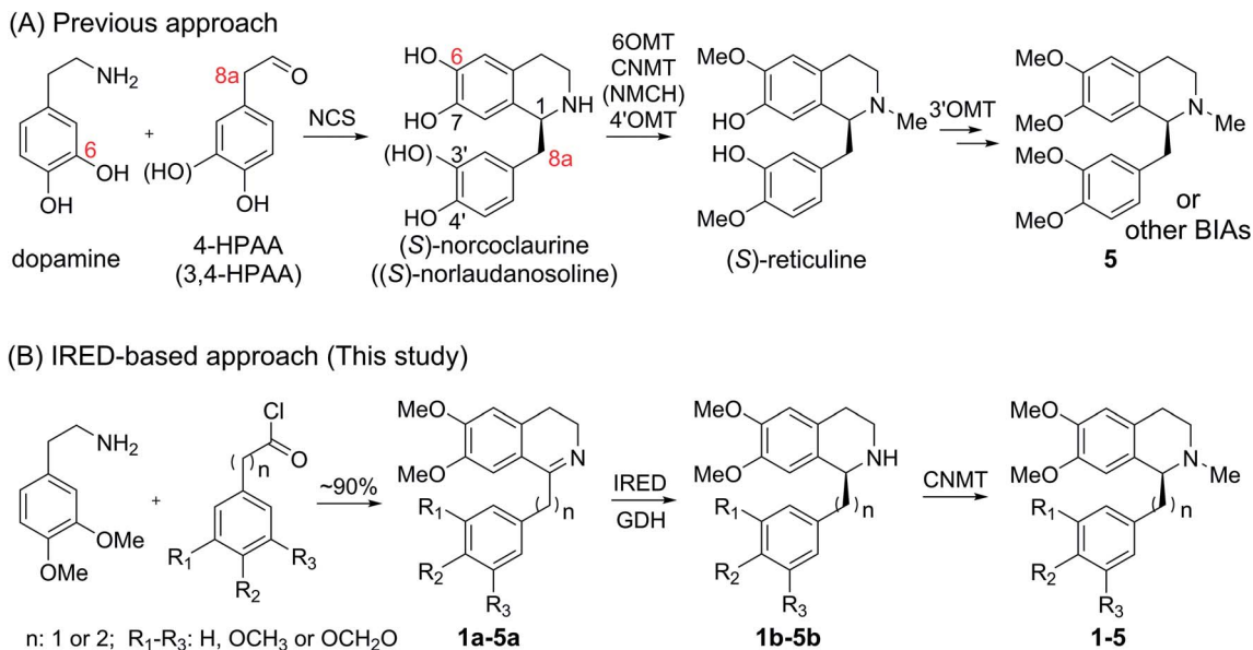
Scheme 2 Approaches for plant TH1QA biosynthesis.
