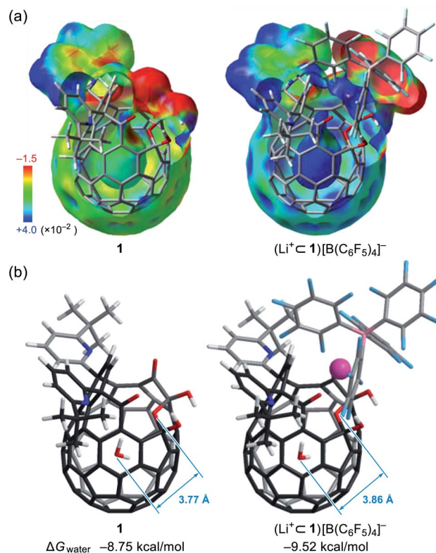
Fig. 8 (a) Electrostatic potential maps inside 1 and (\text{Li}^+\text{C}1)[\text{B}(\text{C}_6\text{F}_5)_4]^- (MP2/6-31G(d,p)//M06-2X/6-31G(d,p)). (b) Global minimum structures of \text{H}_2\text{O}@1 and (\text{Li}^+\text{C}1)[\text{B}(\text{C}_6\text{F}_5)_4]^- (M06-2X/6-31G(d,p), 298 K).
