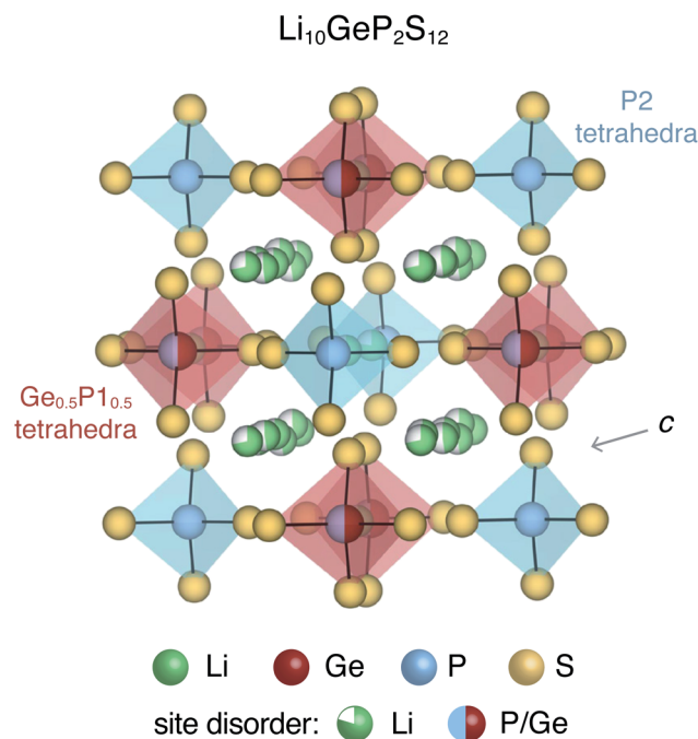
Fig. 1 Tetragonal crystal structure of \text{Li}_{10}\text{GeP}_2\text{S}_{12} contains \text{P}_2\text{S}_4 tetrahedra and (\text{Ge}_{0.5}\text{P}_{1.0.5})_4 tetrahedra with partially occupied Li sites in the c -axis channels and in the a - b plane bridging sites. The S sub-lattice and P2 sites are fully occupied.
